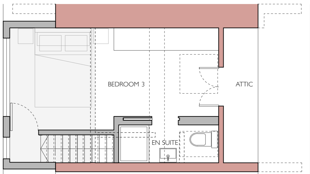
PROPOSED ATTIC PLAN
