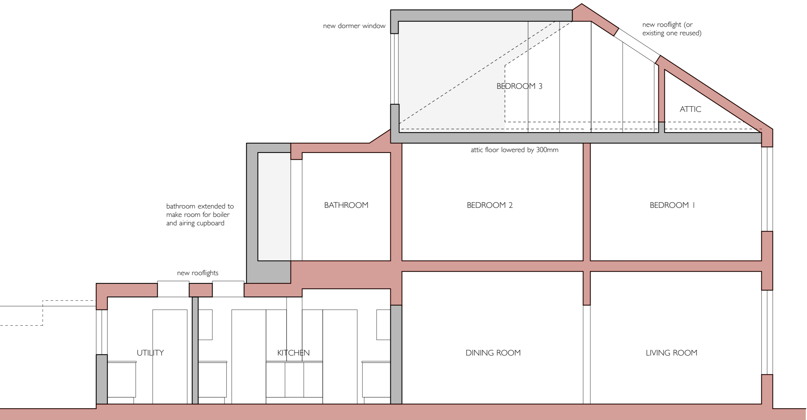
PROPOSED SECTION
