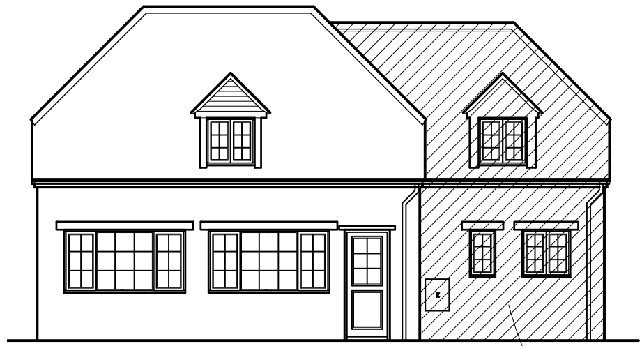
FRONT (EAST)
