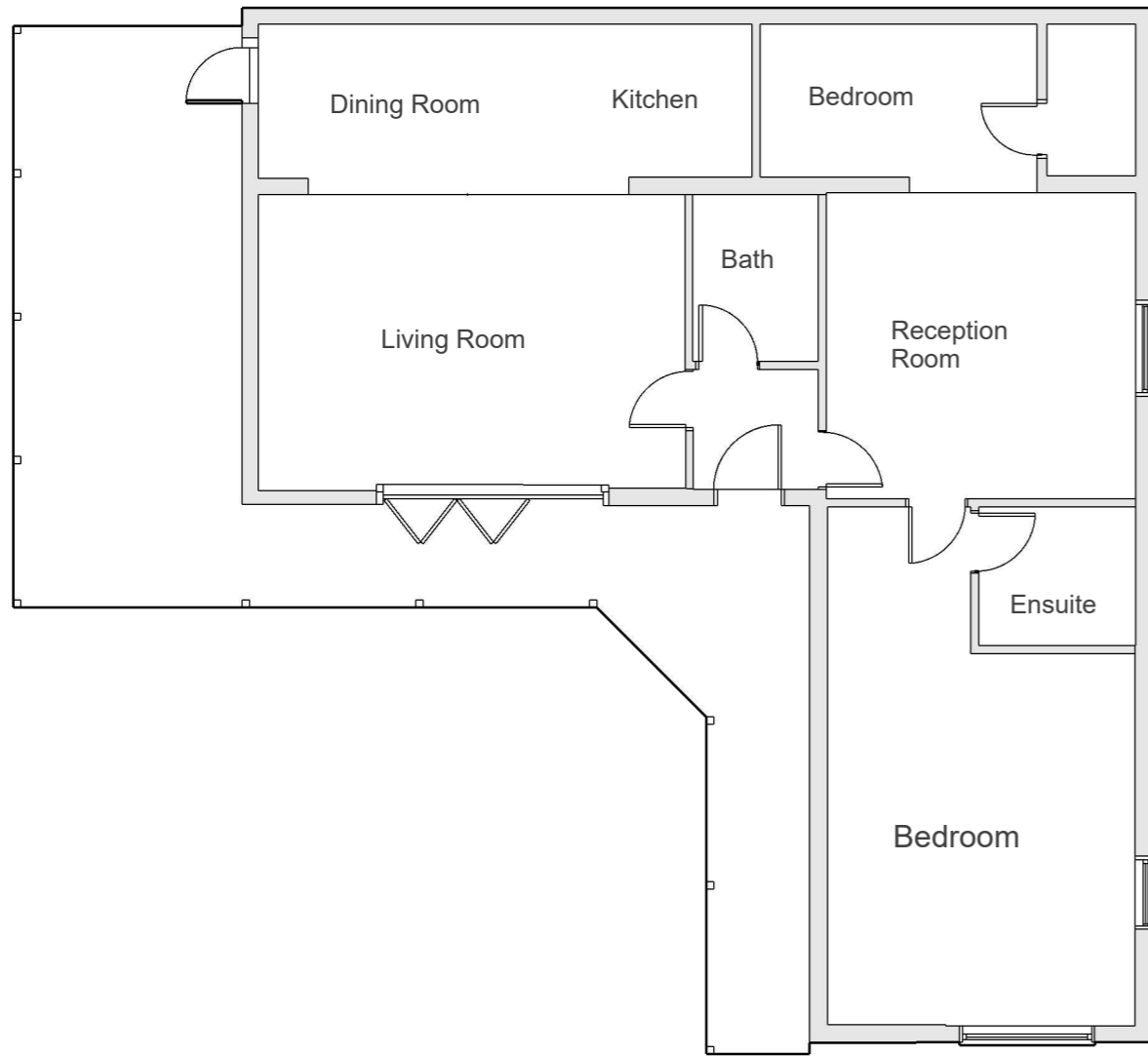
Ground Floor - Existing
