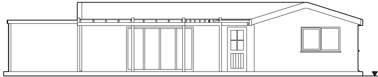
South Elevation
