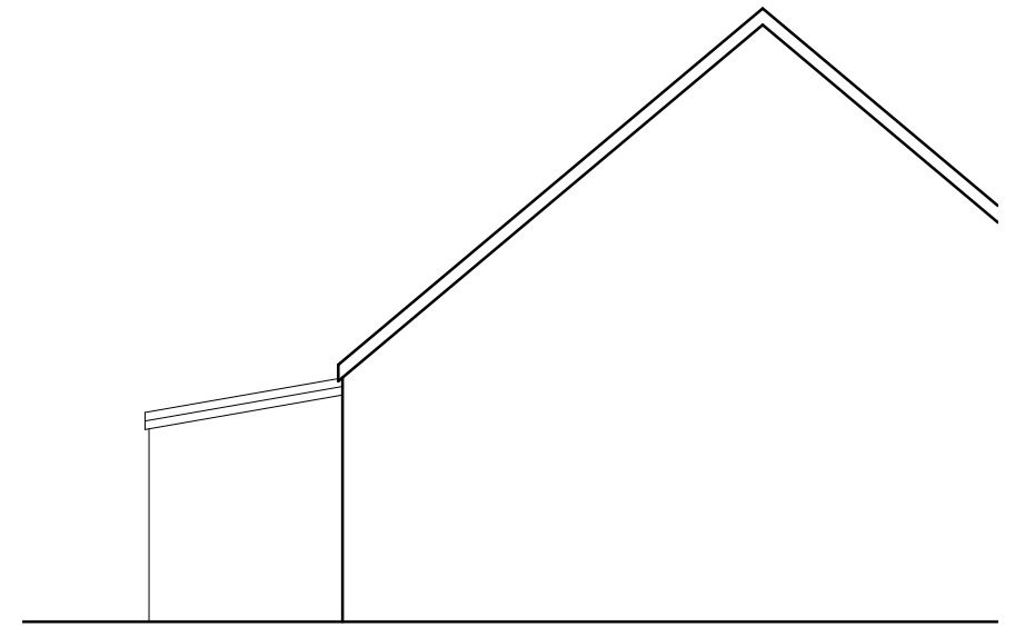
Existing North East Elevation Scale 1.100
