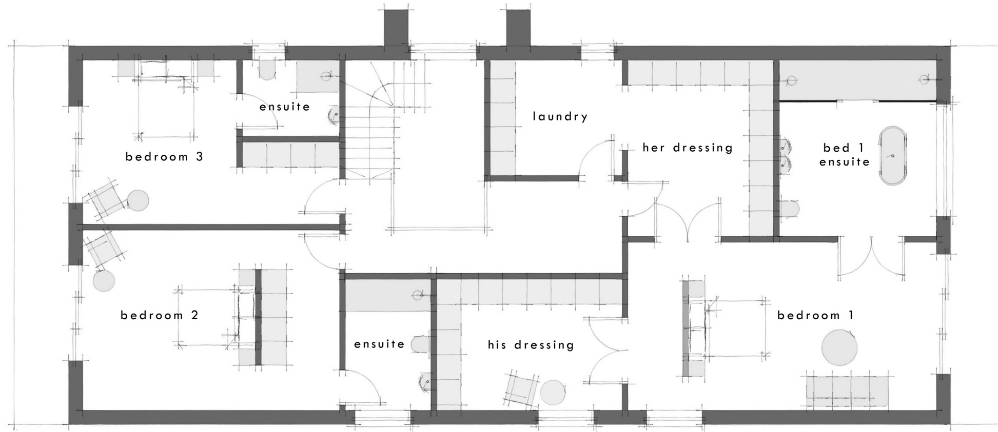
proposed first floor plan dwelling 2 scale 1:100
