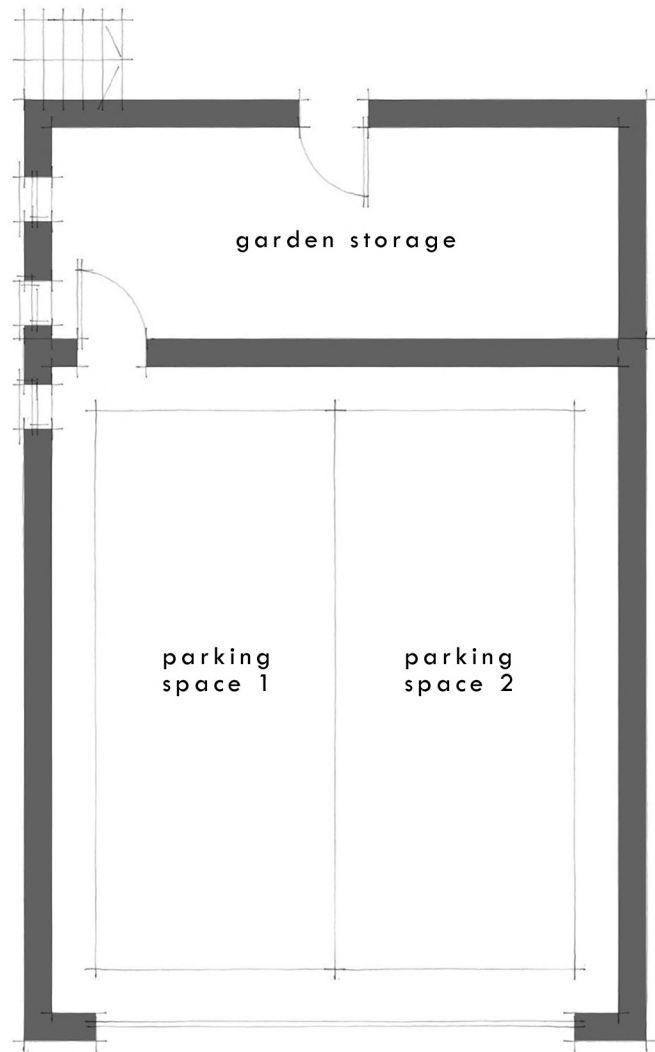
proposed garage ground floor plan scale 1:100
