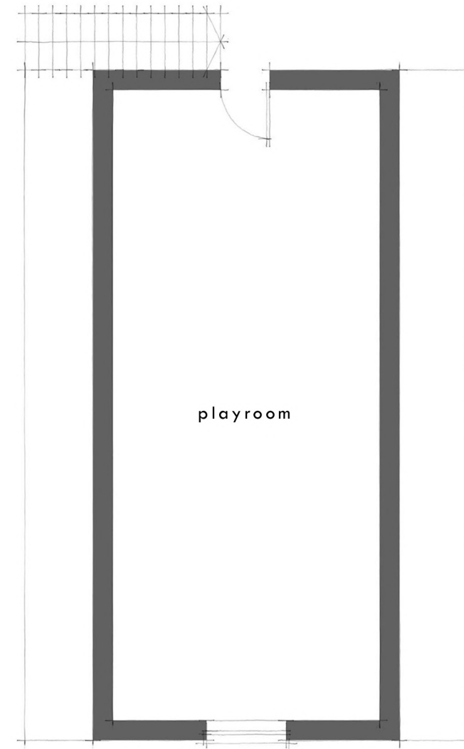
proposed garage loft space scale 1:100
