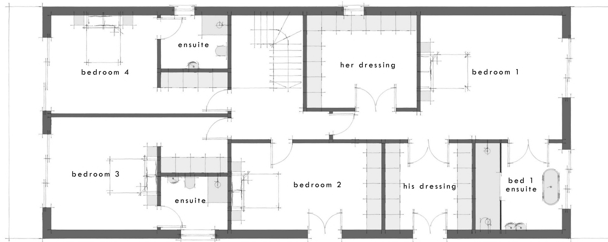
proposed first floor plan dwelling 2 scale 1:100
