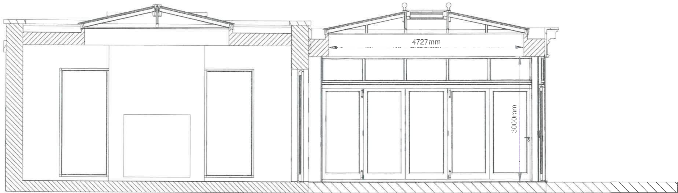
Proposed Section Thru
