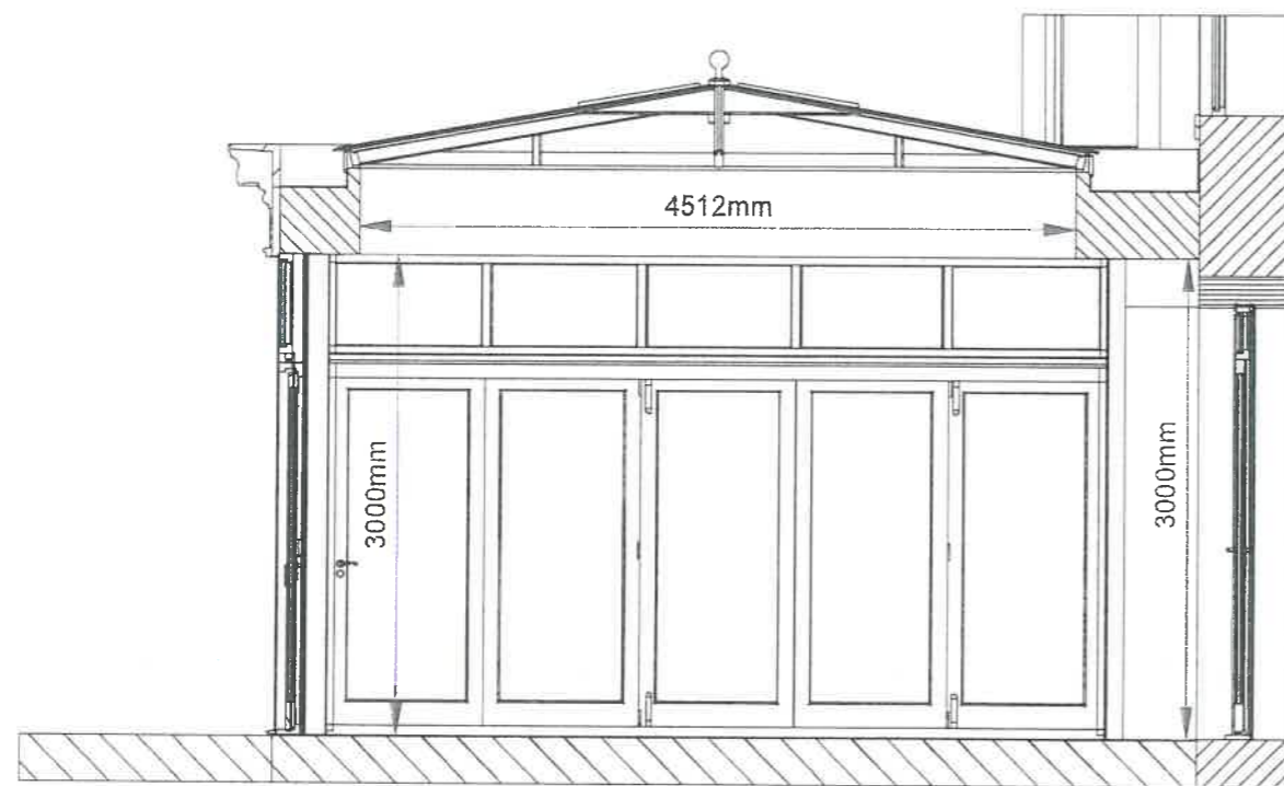
Proposed Section Thru
