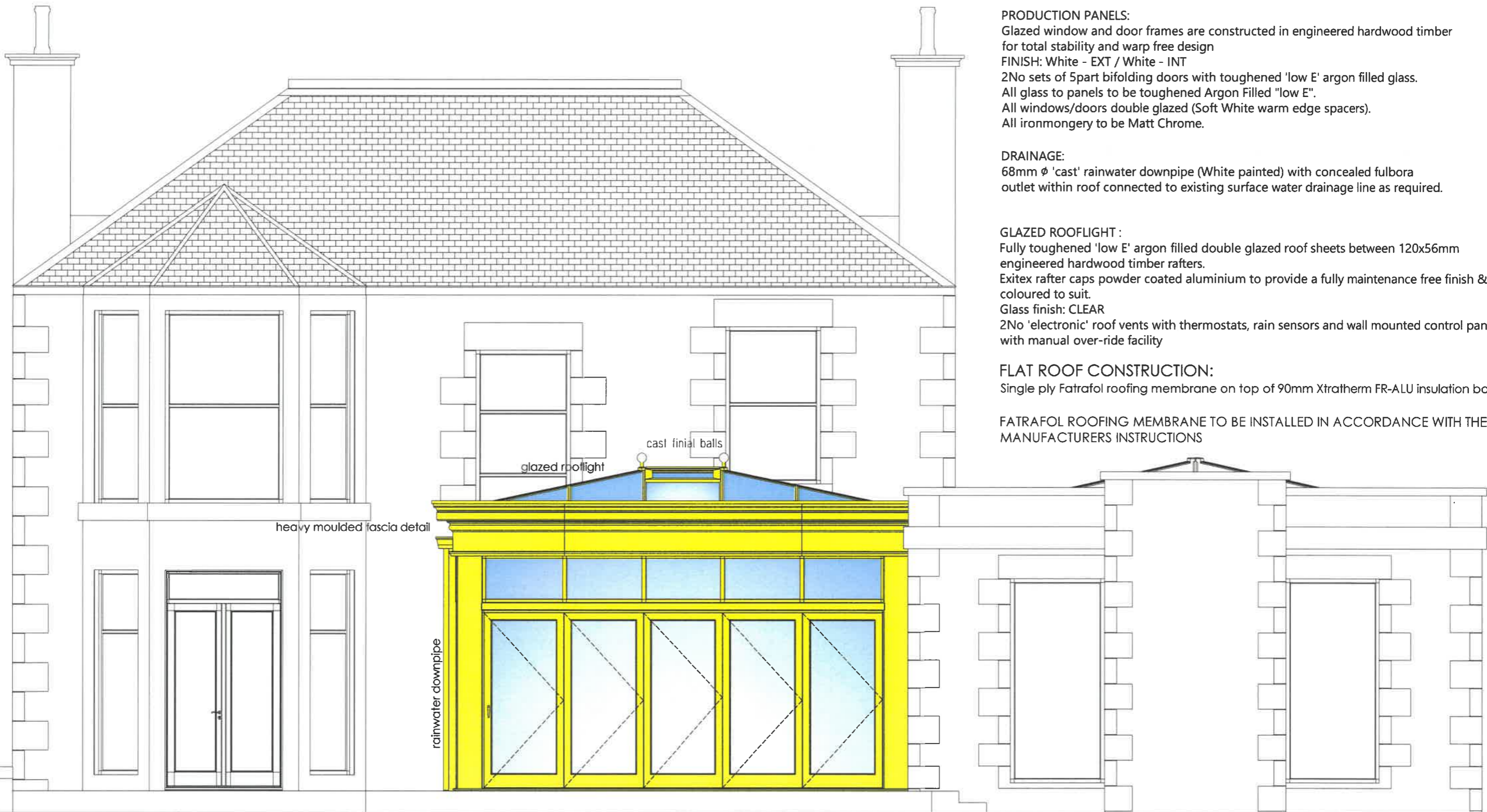
Proposed South Elevation scale : 1:50
