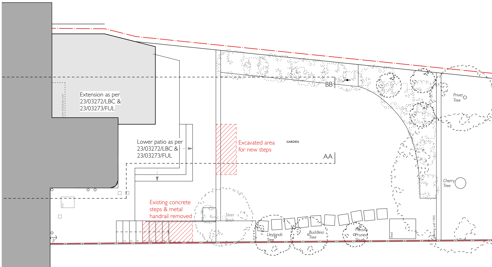
1 Existing Rear Garden Plan Scale: 1:100
