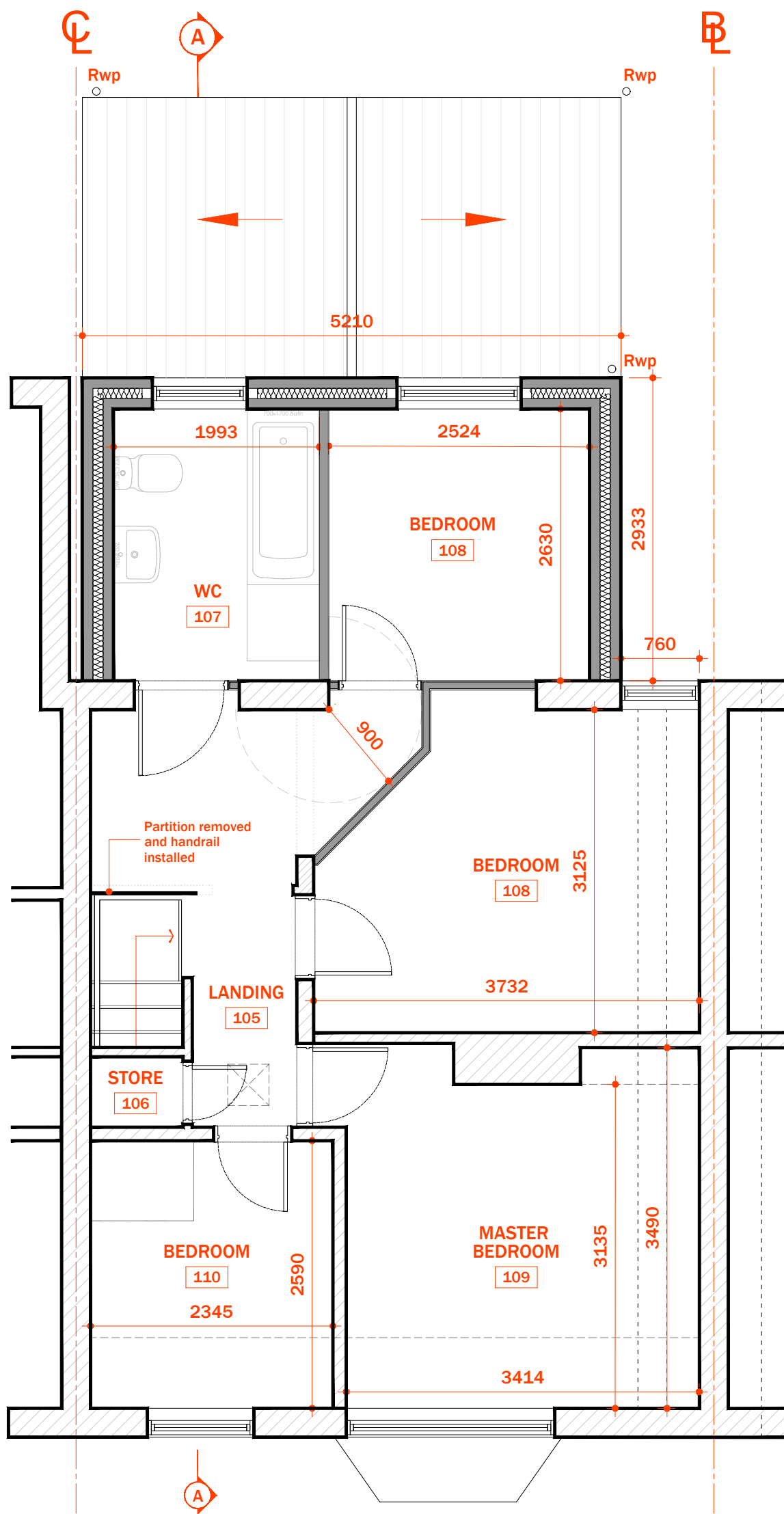
202 PROPOSED FIRST FLOOR PLAN 1:100 @ A3
