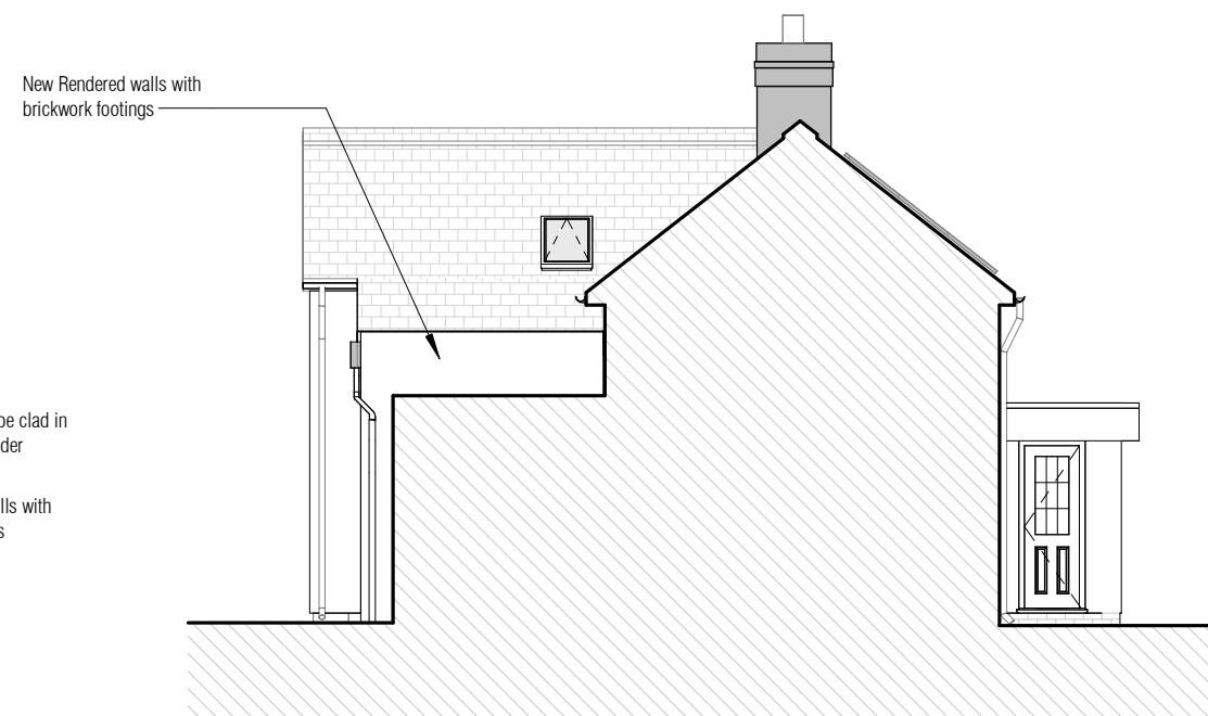
Side Elevation 2 - Proposed
