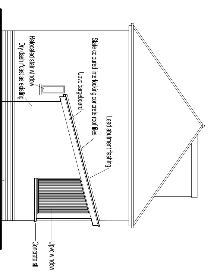
PROPOSED SIDE (SE) ELEVATION 1 : 100 @ A3
