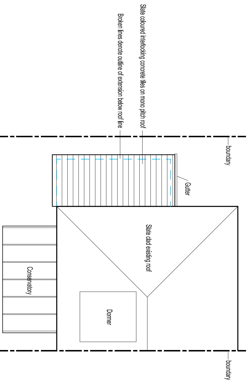
ROOF PLAN 1 : 100 @ A3
