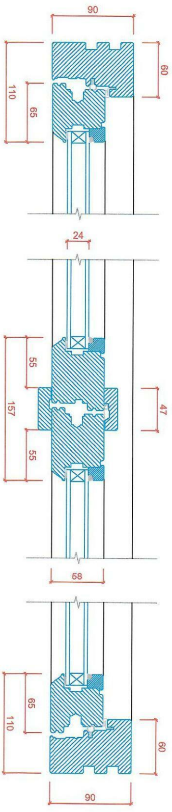
CASEMENT CROSS SECTION 'A-A'
