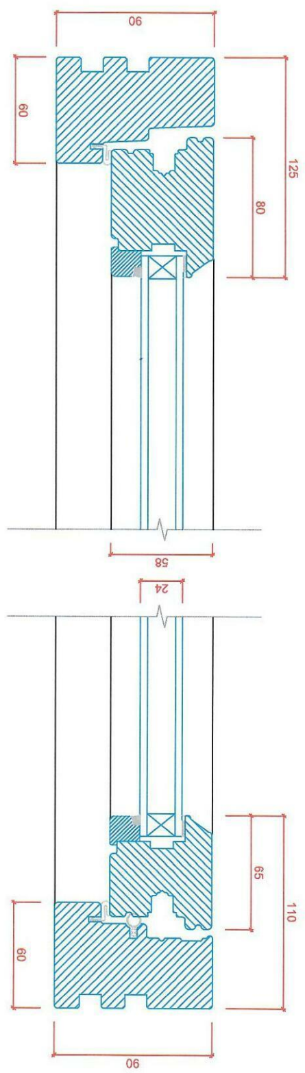
CASEMENT CROSS SECTION A-A'
