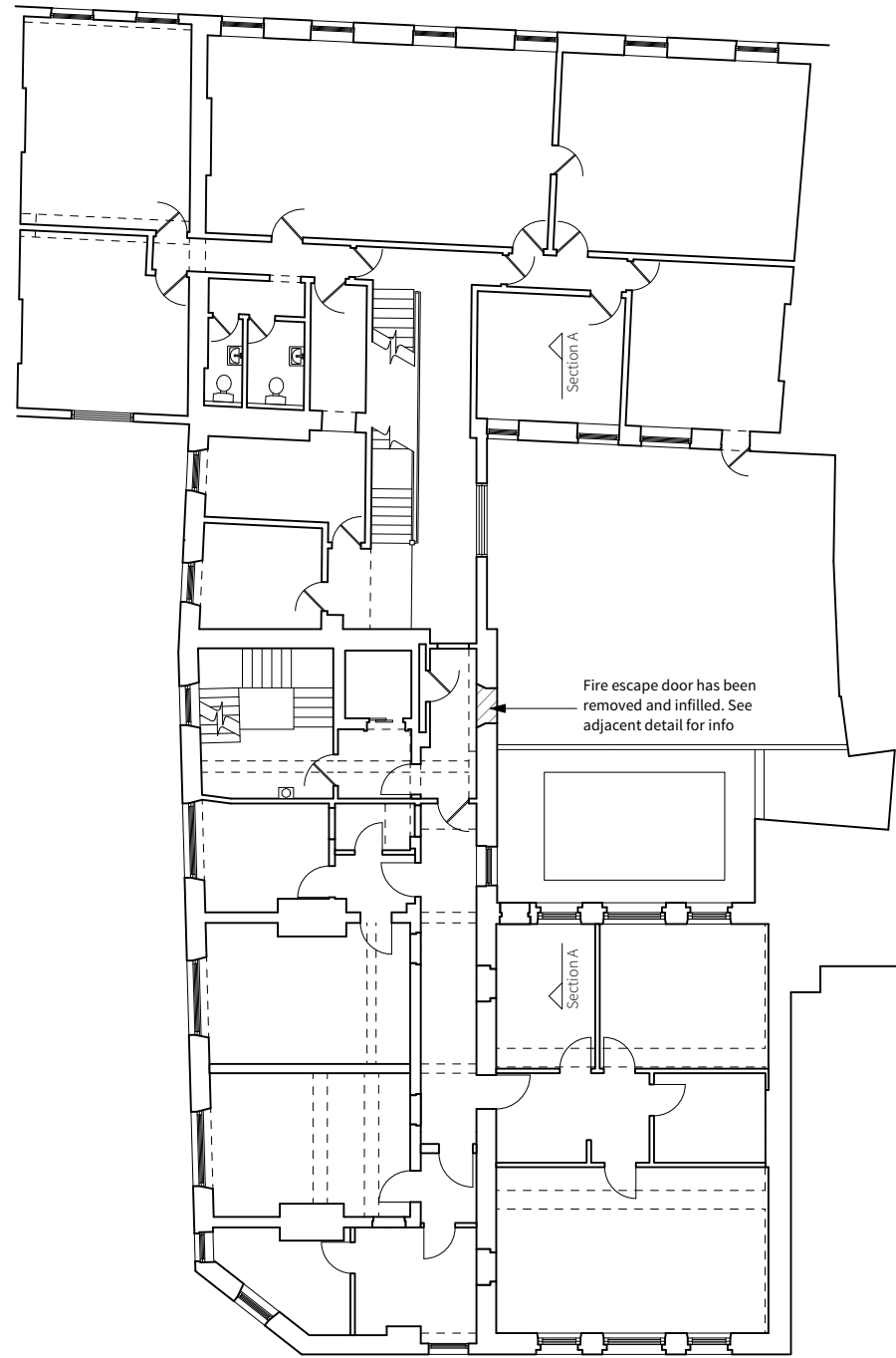
Existing First Floor Plan 1:200 @A3
