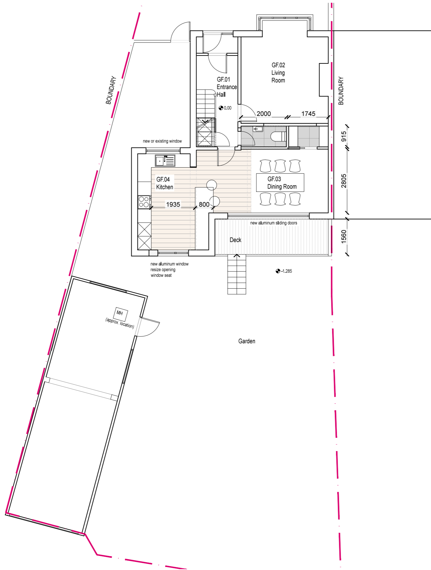
1 GROUND FLOOR AS PROPOSED (10)05 1:100
