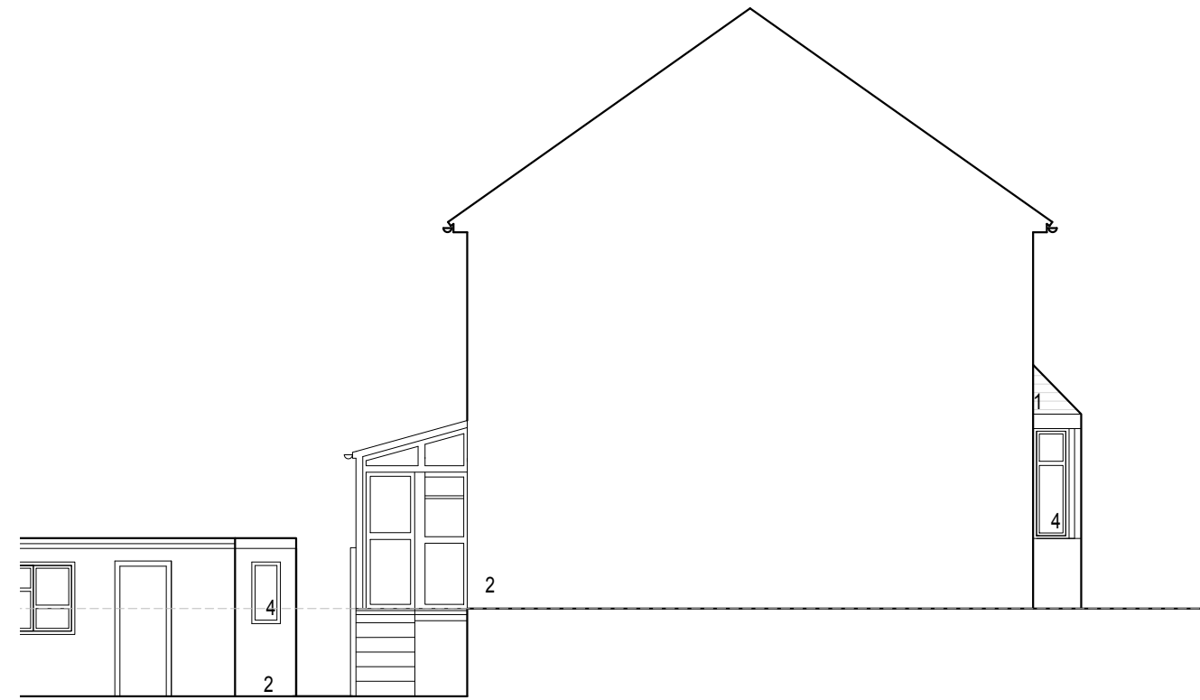
4 NORTH ELEVATION AS EXISTING (10)03 1:100
