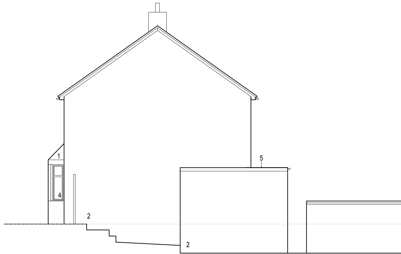
3 SOUTH ELEVATION AS EXISTING (10)03 1:100
