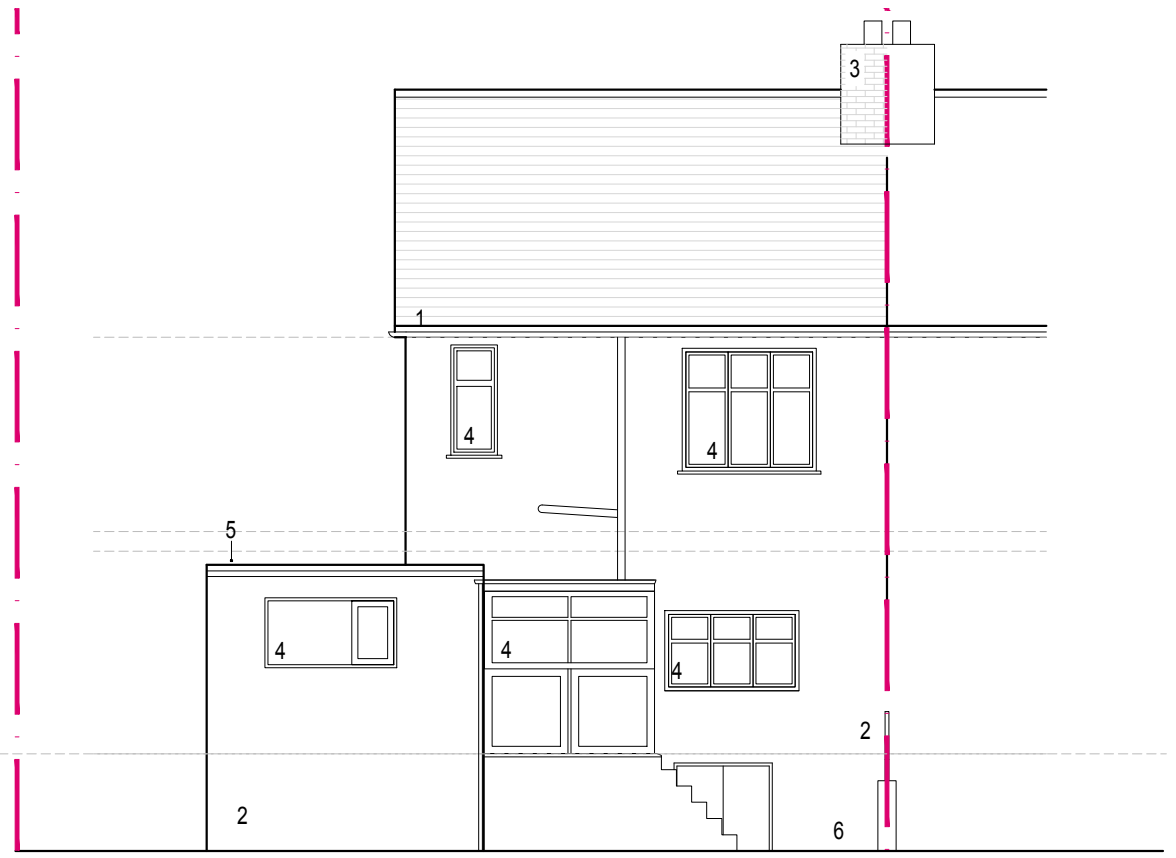
2 REAR ELEVATION AS EXISTING (10)03 1:100
