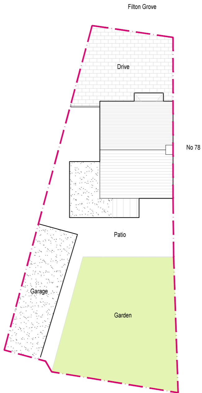
2 BLOCK PLAN AS EXISTING (10)01 1:200
