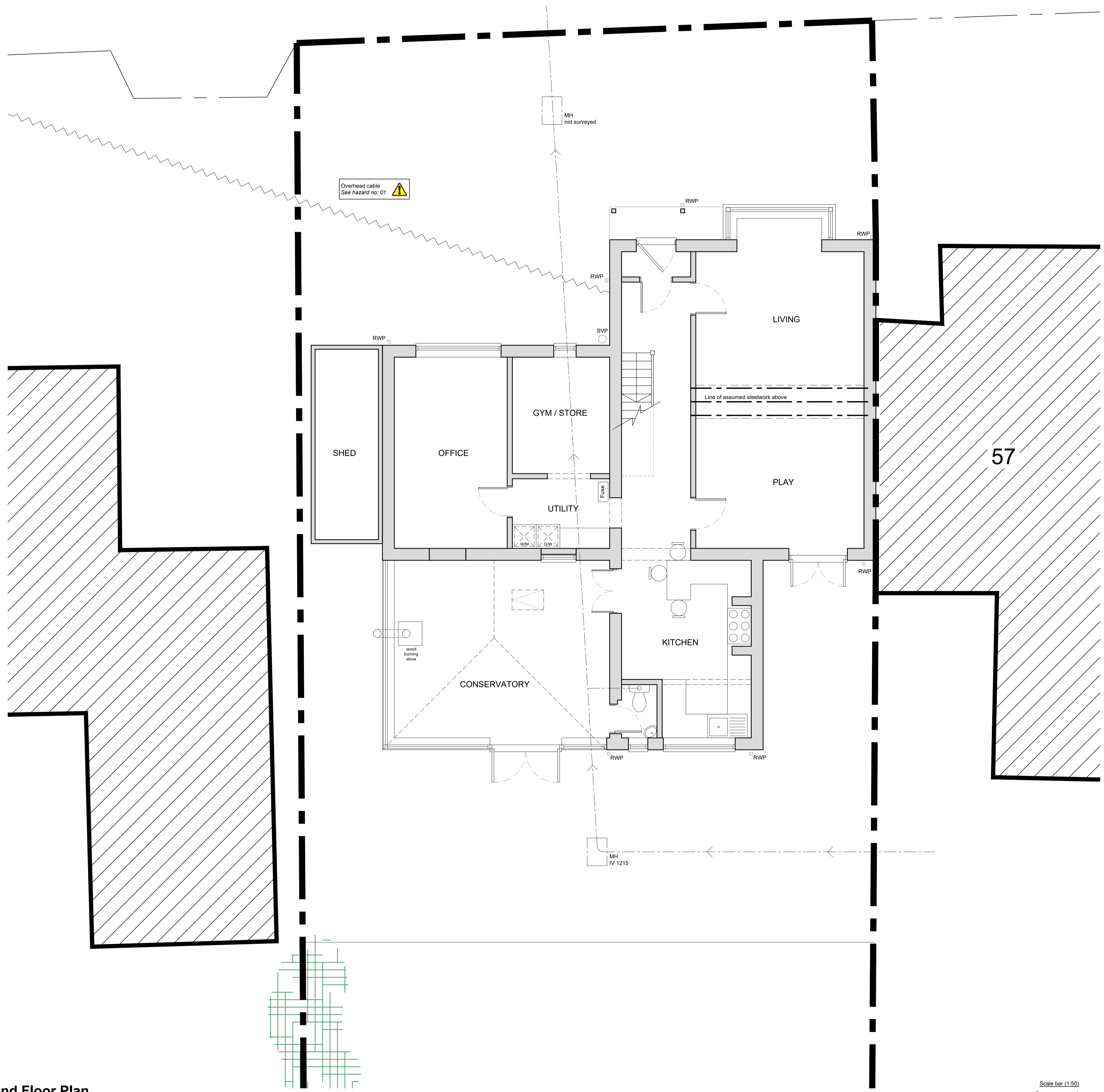
Existing Ground Floor Plan Scale 1:50 @ A1
