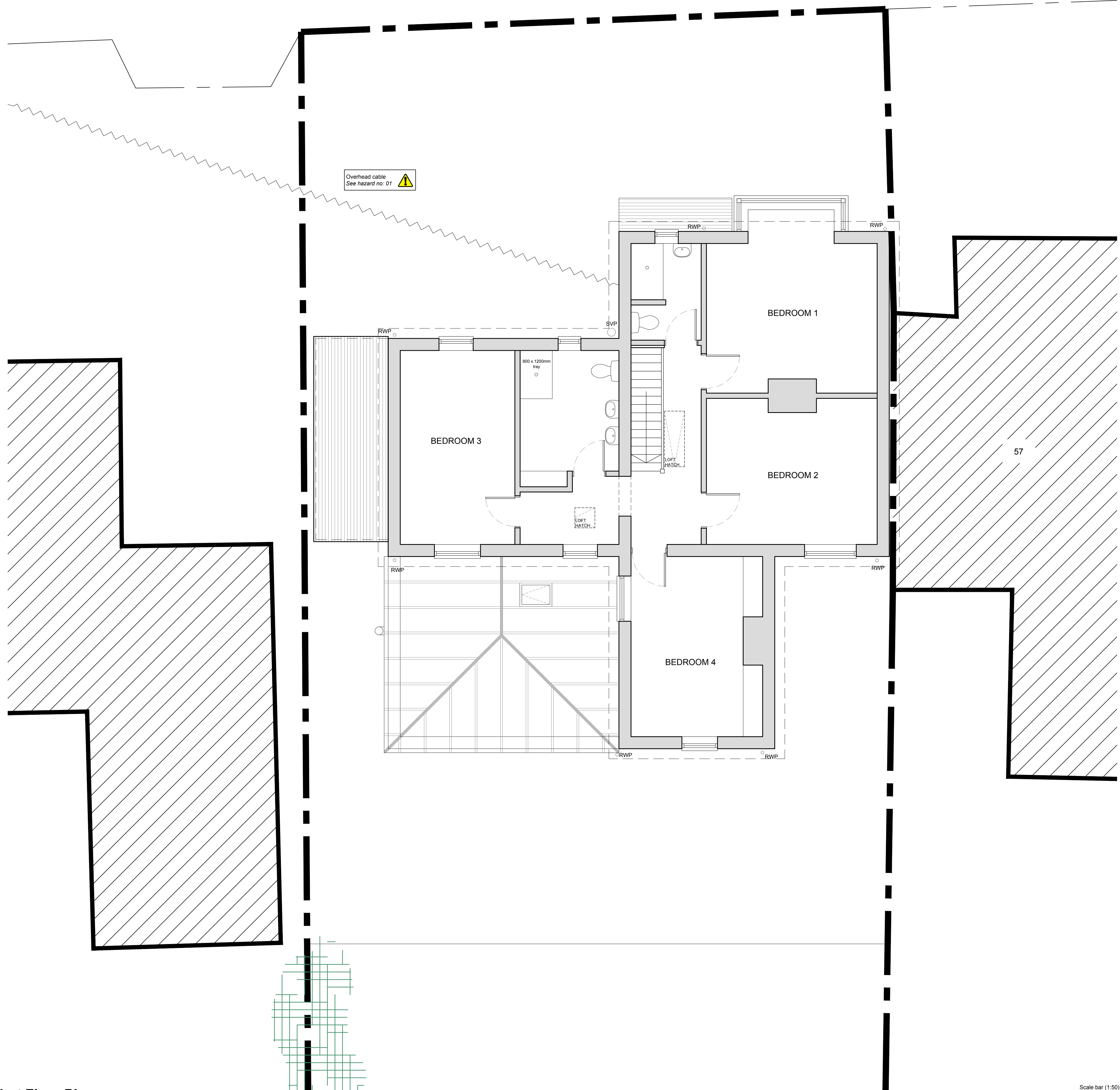
Existing First Floor Plan Scale 1:50 @ A1
