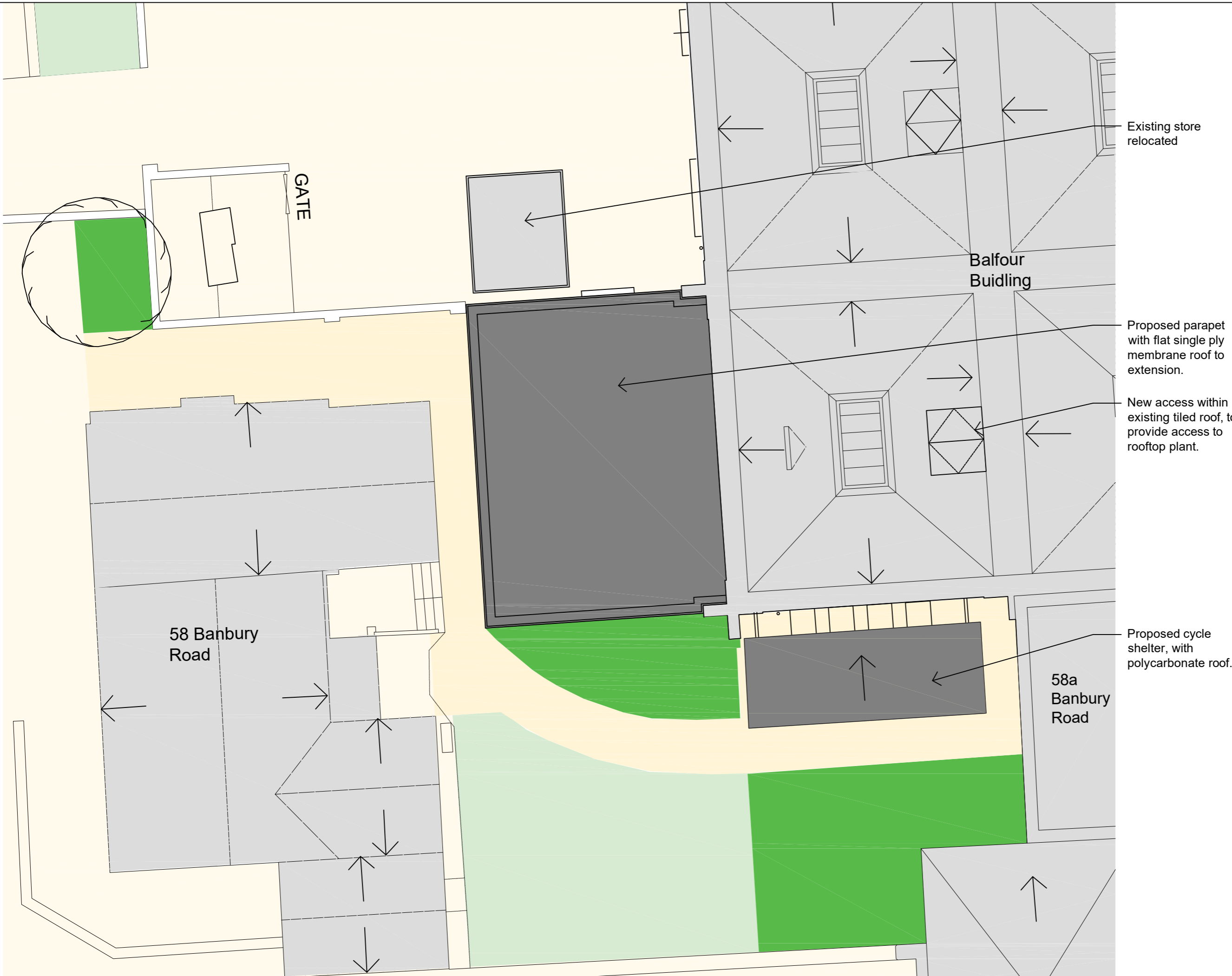
1 PROPOSED ROOF PLAN 1:100
