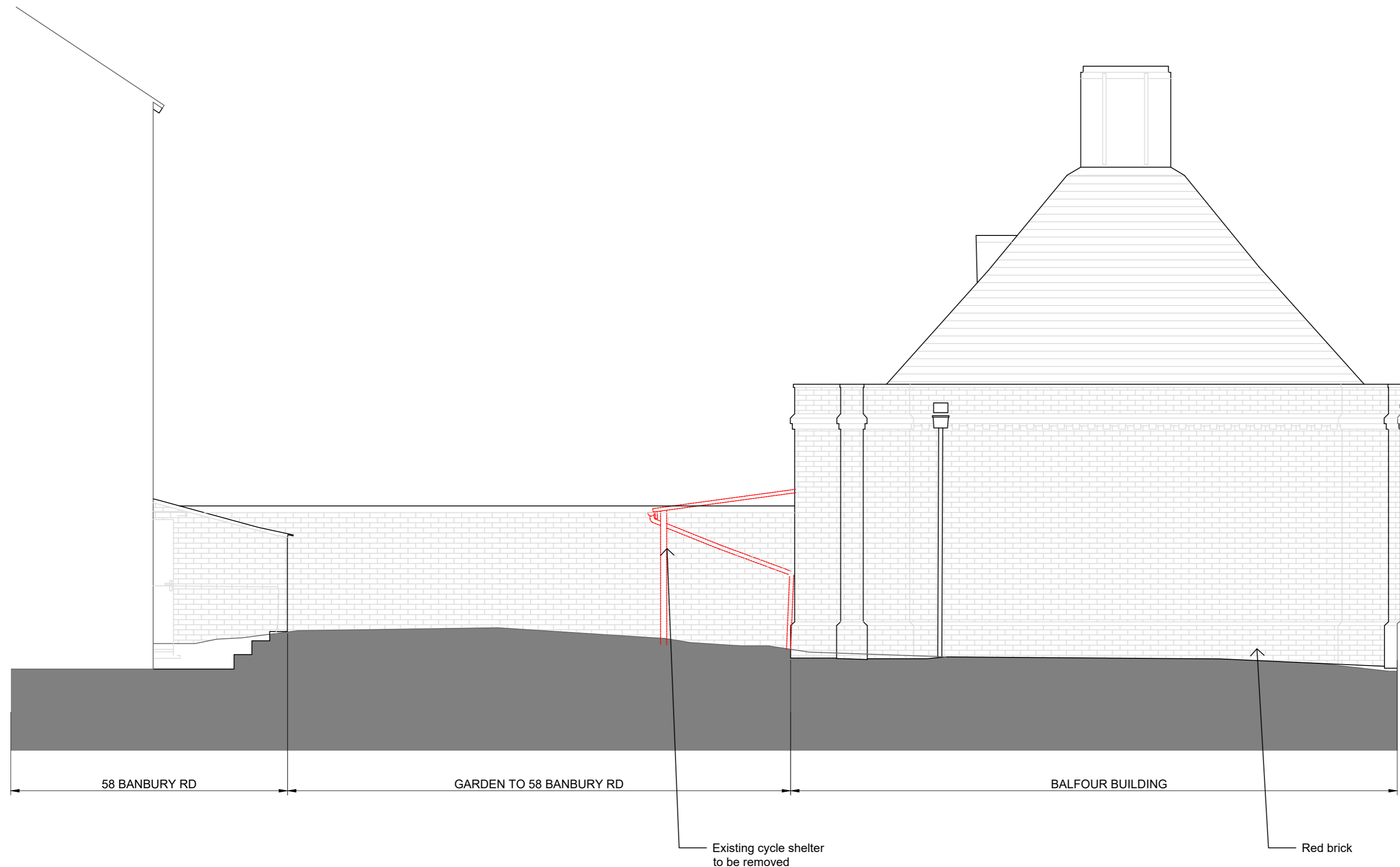
⑦ Existing South Elevation 1:50
