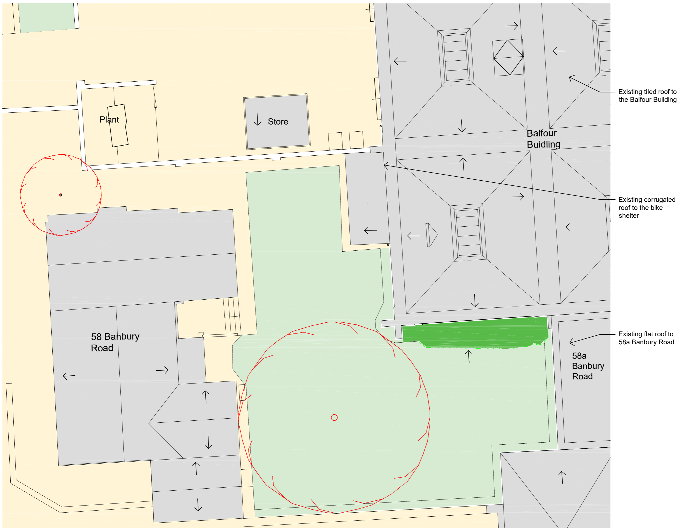
4 EXISTING ROOF PLAN 1:100
