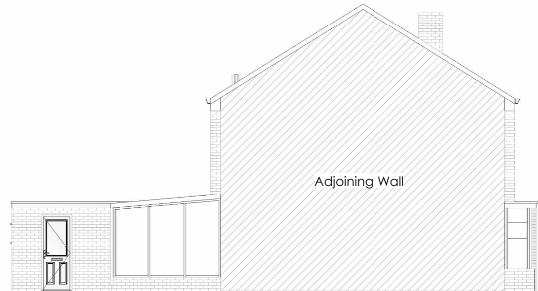
EXISTING SIDE B ELEVATION
