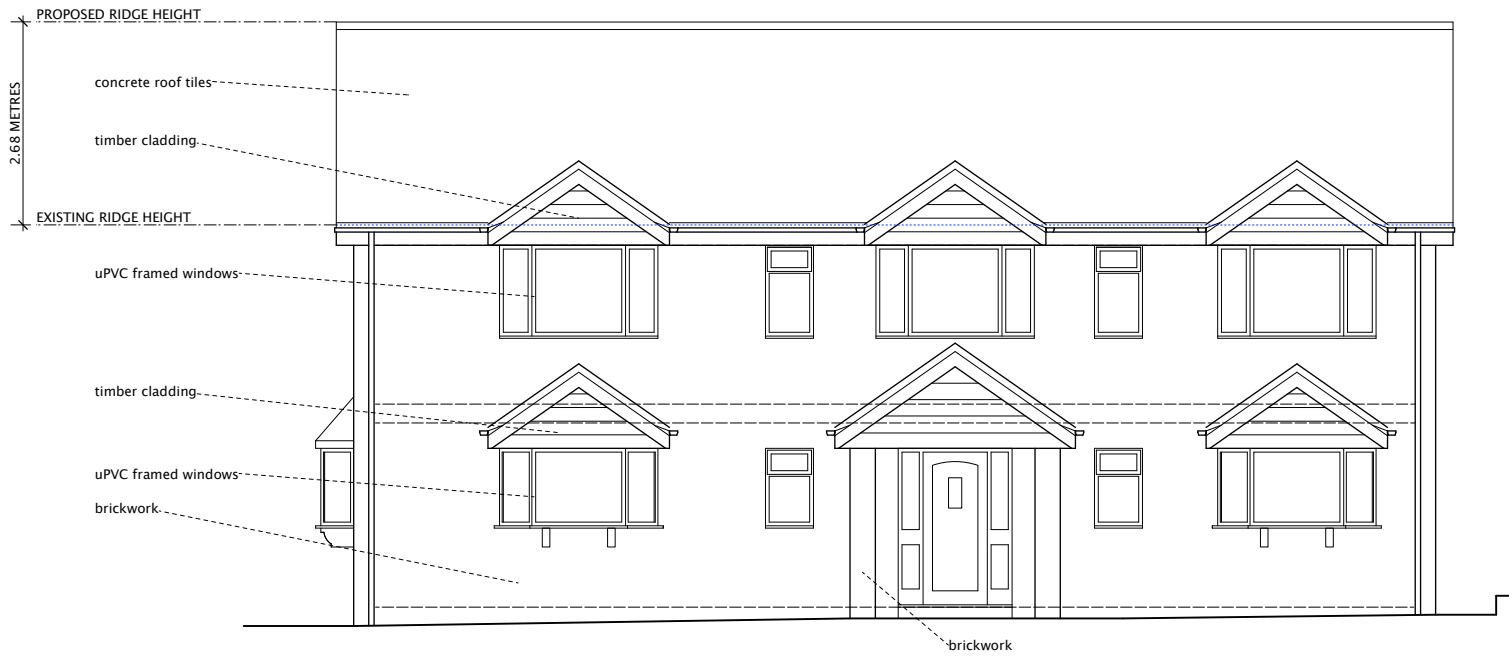
EAST ELEVATION
