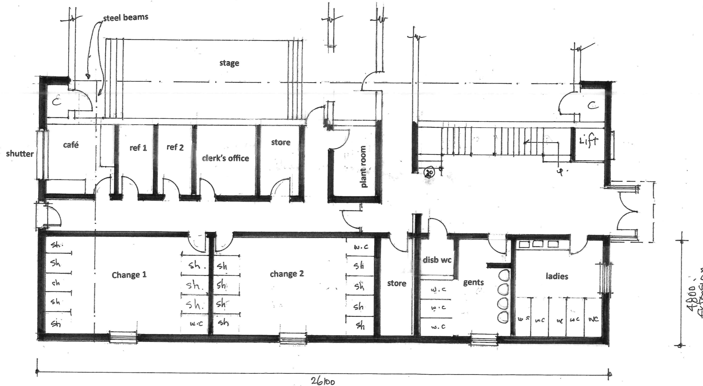
GROUND FLOOR - PROPOSED
