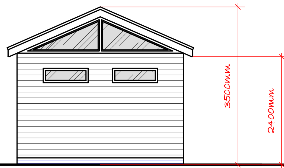
Proposed Side Elevation 1:50
