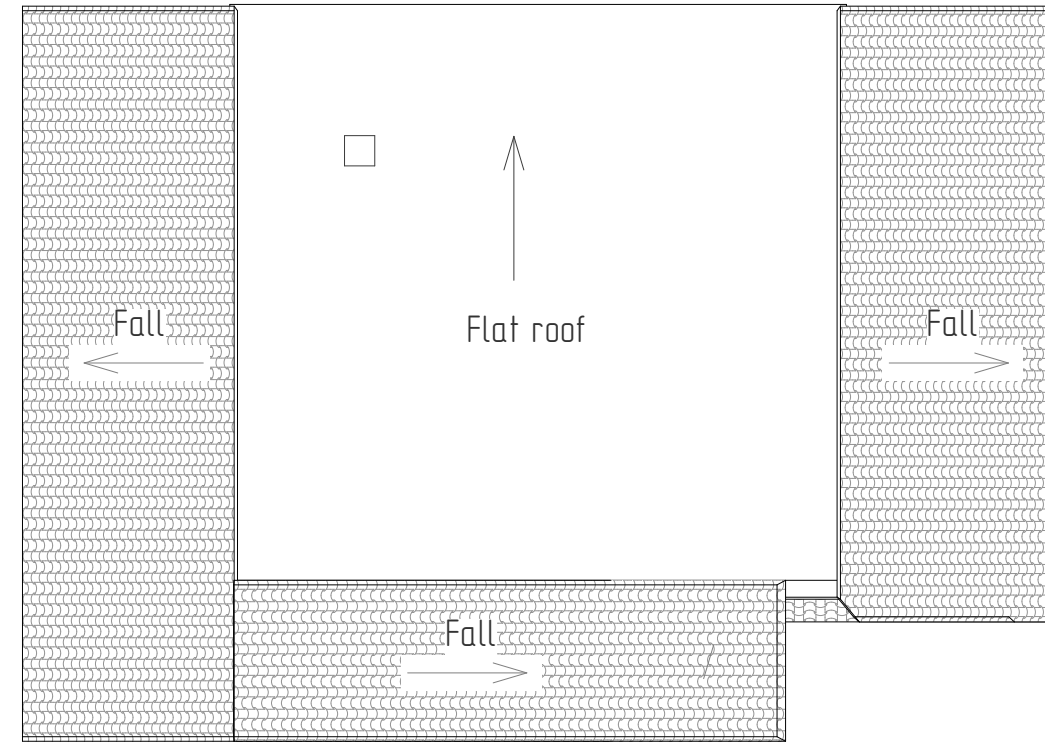
Roof Plan
