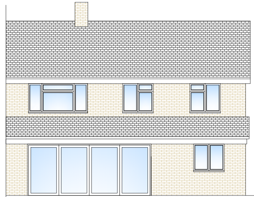
REAR
