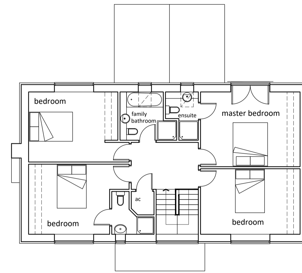
first floor plan 78m 2 gfa
