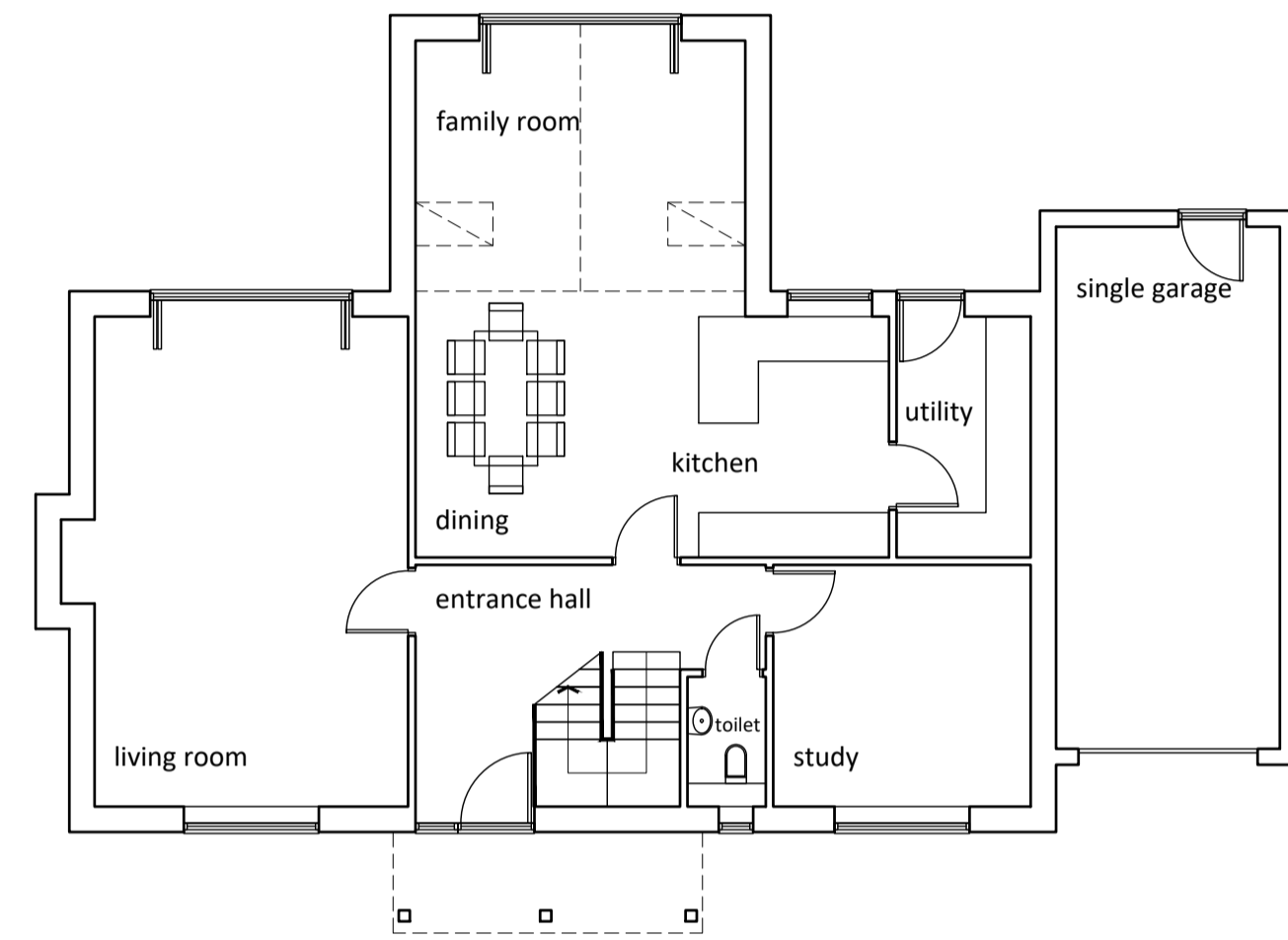
ground floor plan 99m 2 gfa
