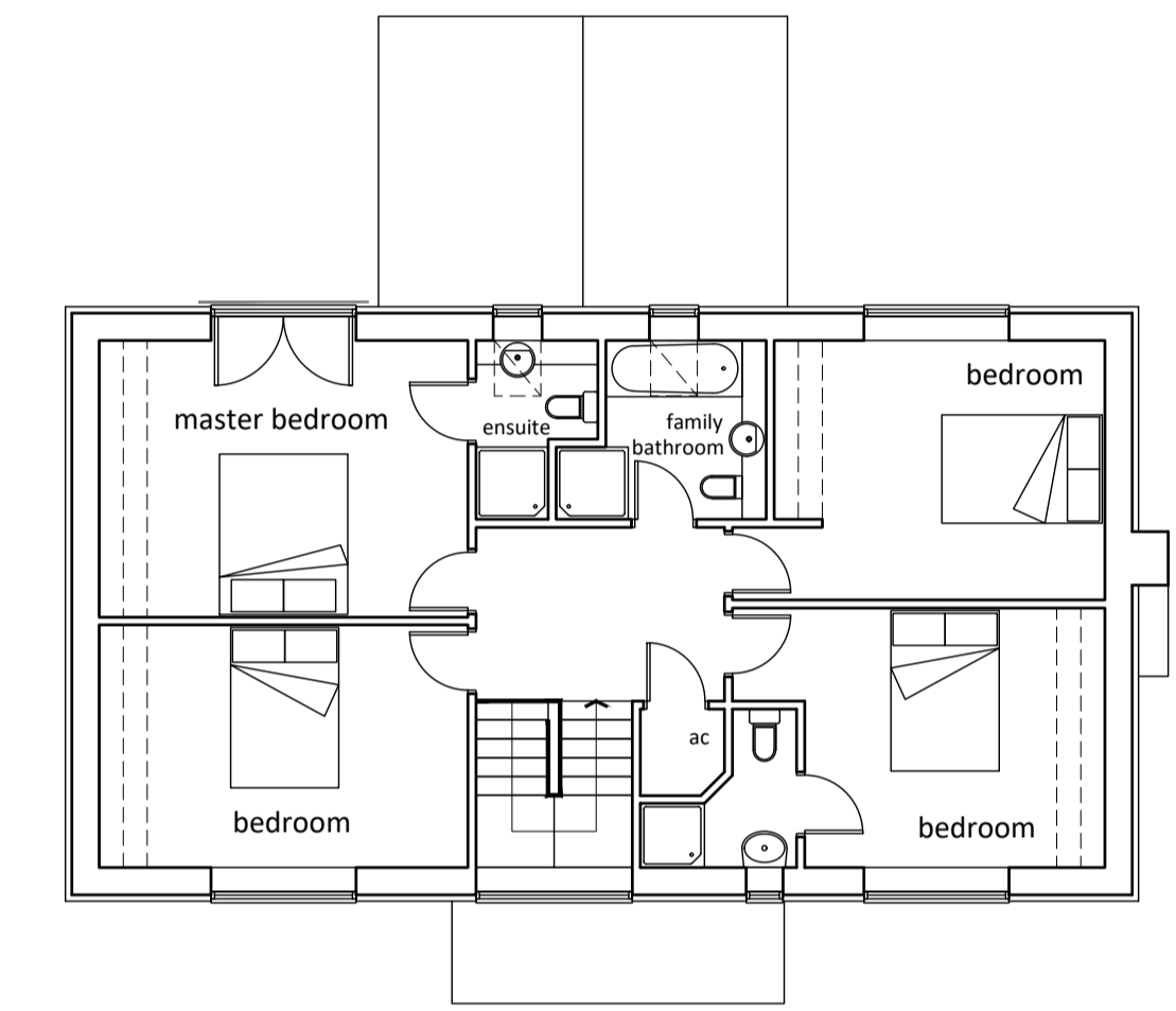
first floor plan 78m 2 gfa
