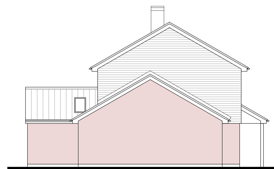
west elevation
