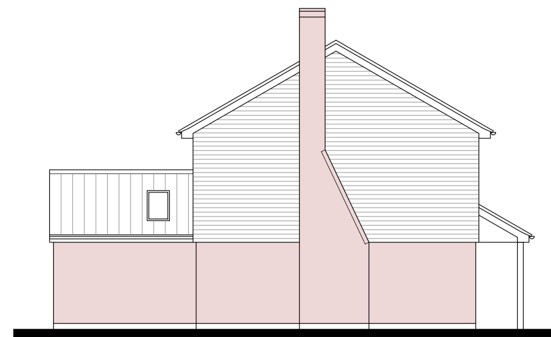
west elevation
