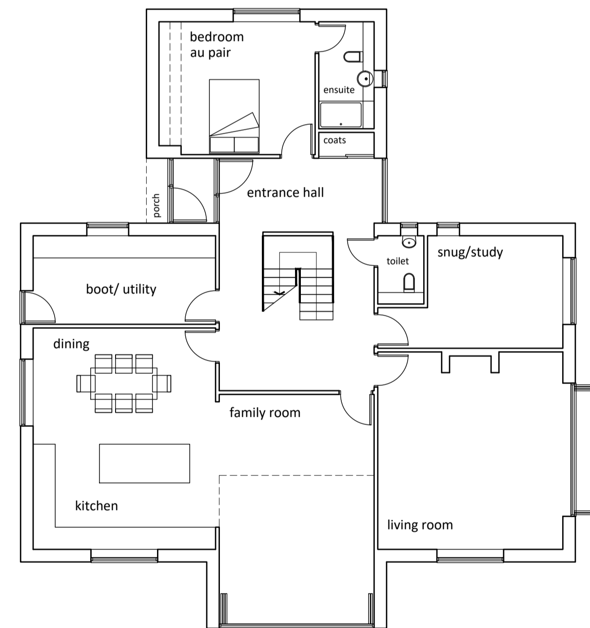
ground floor plan 164m 2 gja
