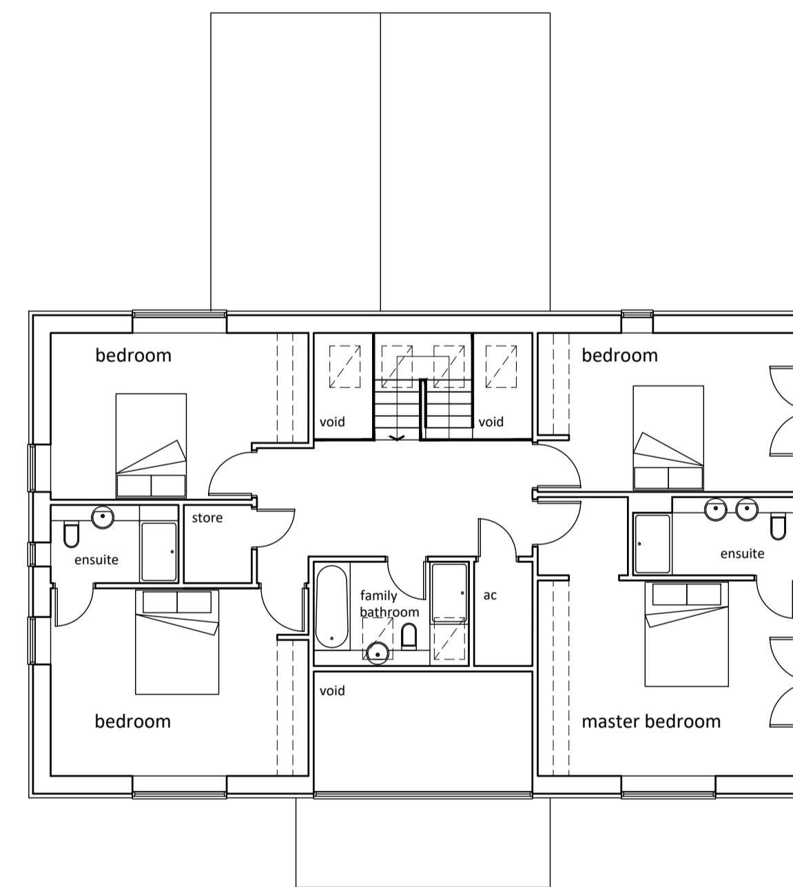
first floor plan 104m 2 gja
