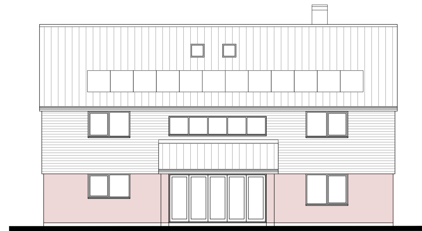
south elevation
