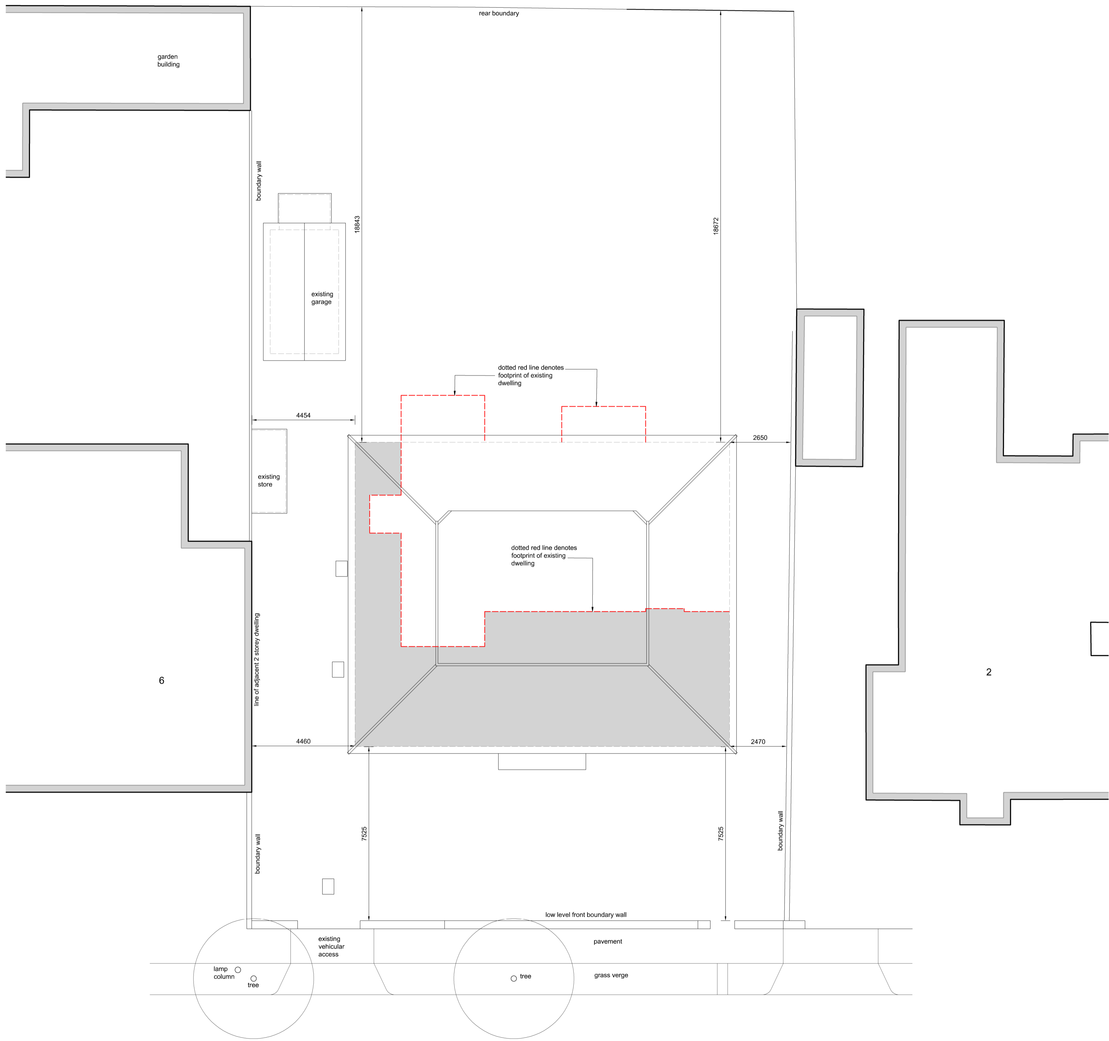
Proposed site layout
