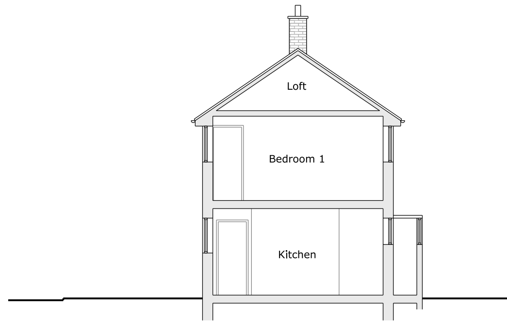
Long Section
