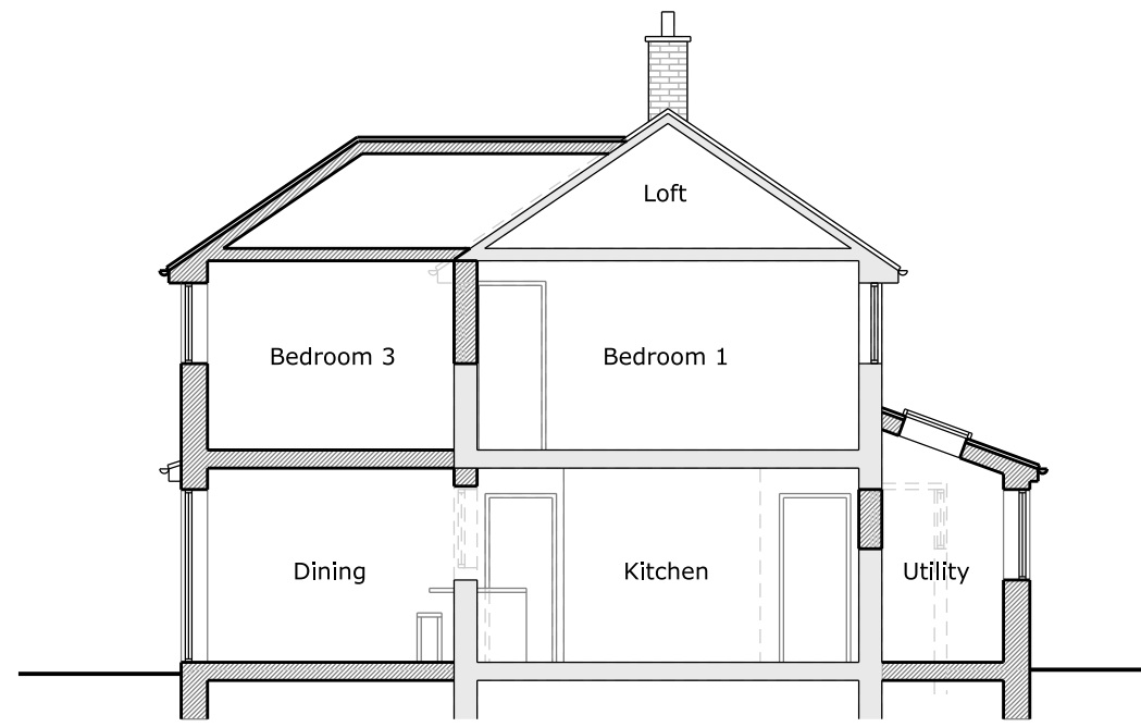
Long Section
