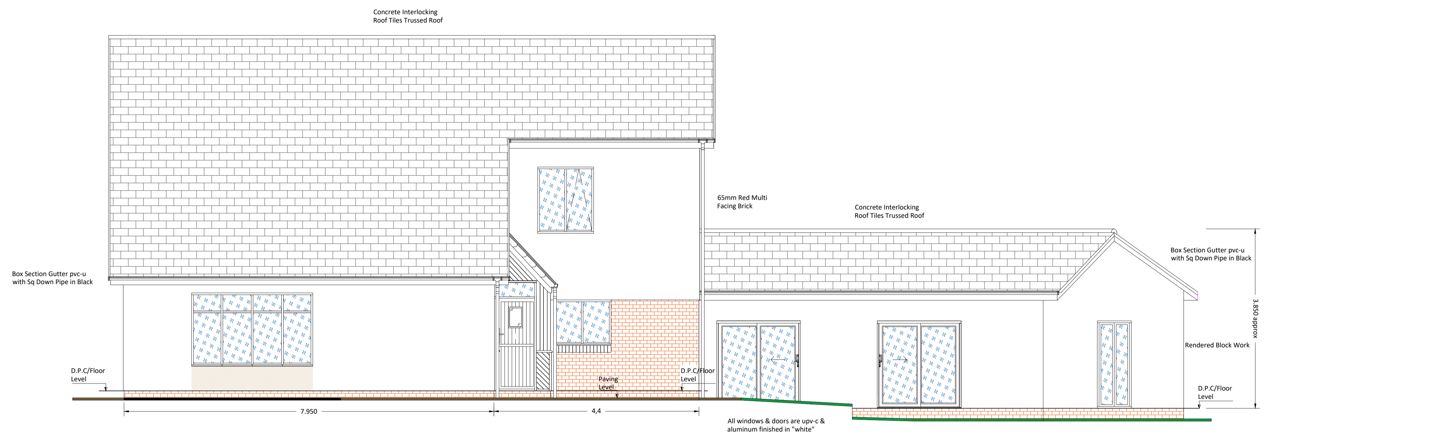
Existing Side (East) Elevation
