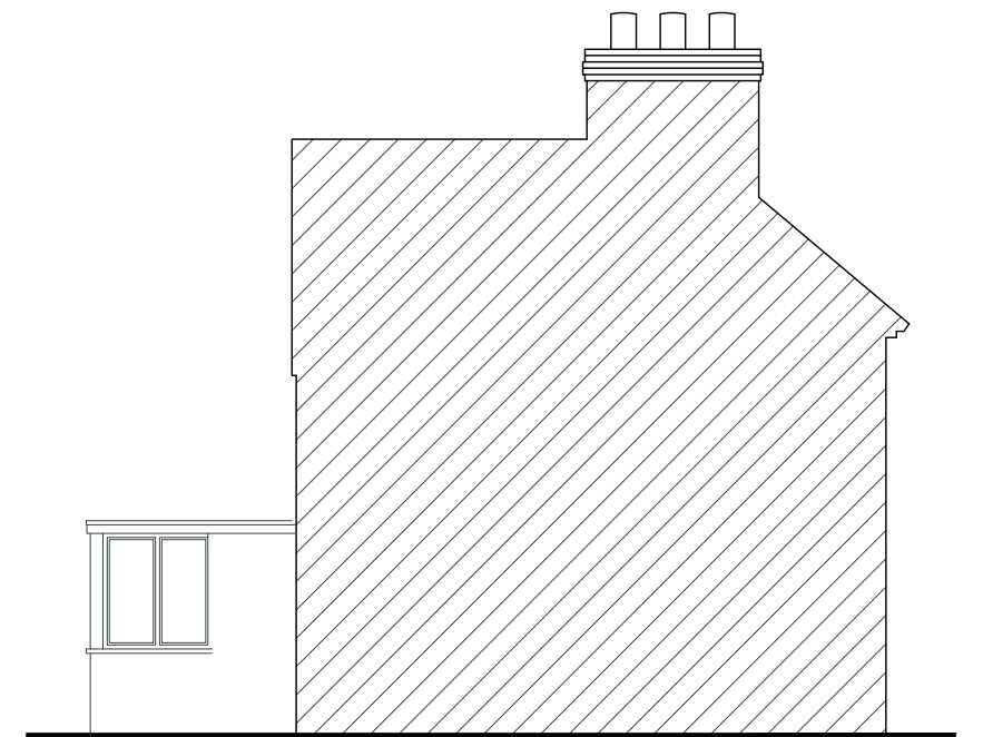
AS EXISTING SIDE (PARTY WALL) ELEVATION 1:100 @ A3
