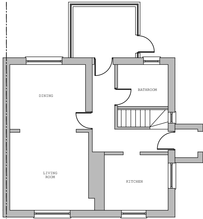
AS EXISTING GROUND FLOORPLAN 1:100 @ A3
