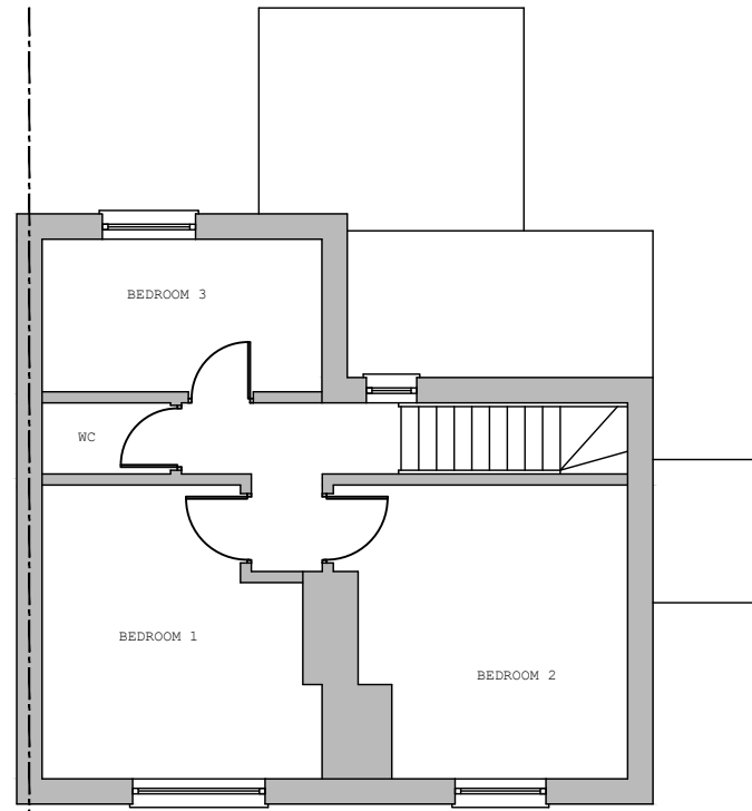
AS EXISTING FIRST FLOORPLAN 1:100 @ A3
