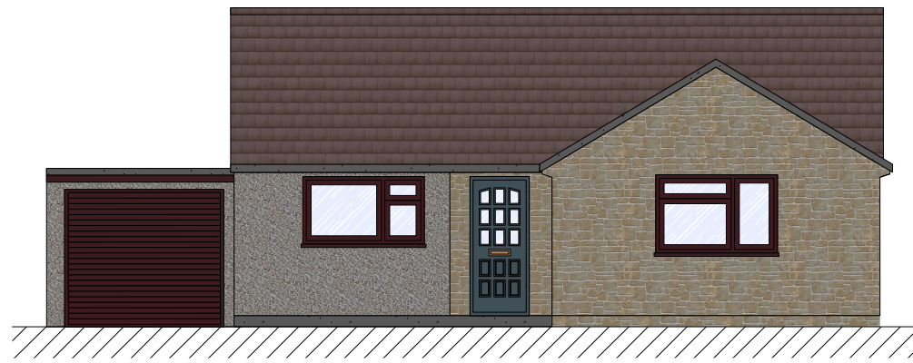
South East Elevation as Existing SCALE 1:100
