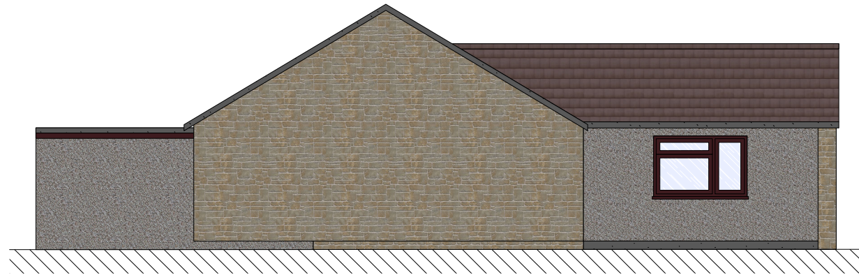
South East Elevation as Existing SCALE 1:100
