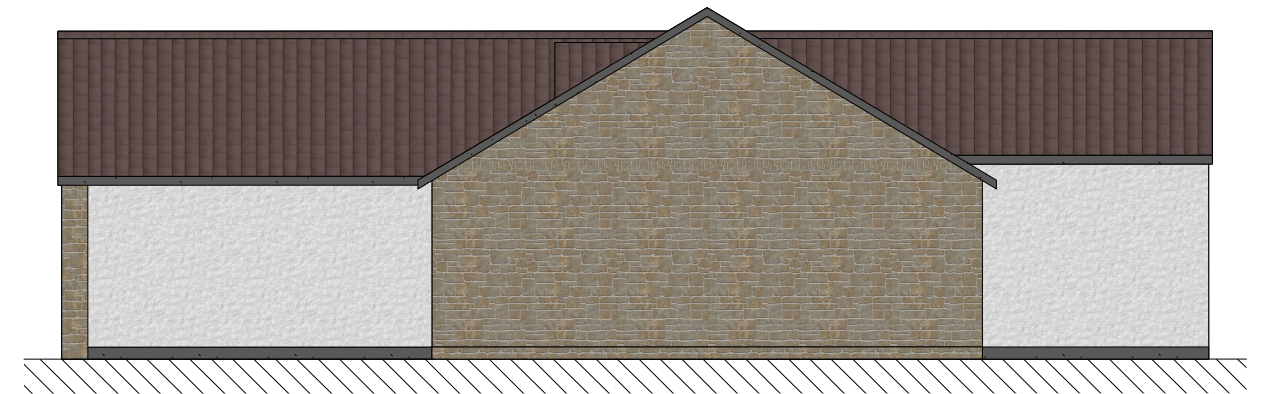
North East Elevation as Proposed SCALE 1:100
