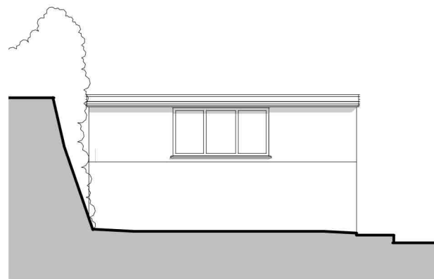
Existing South Elevation 1 : 100
