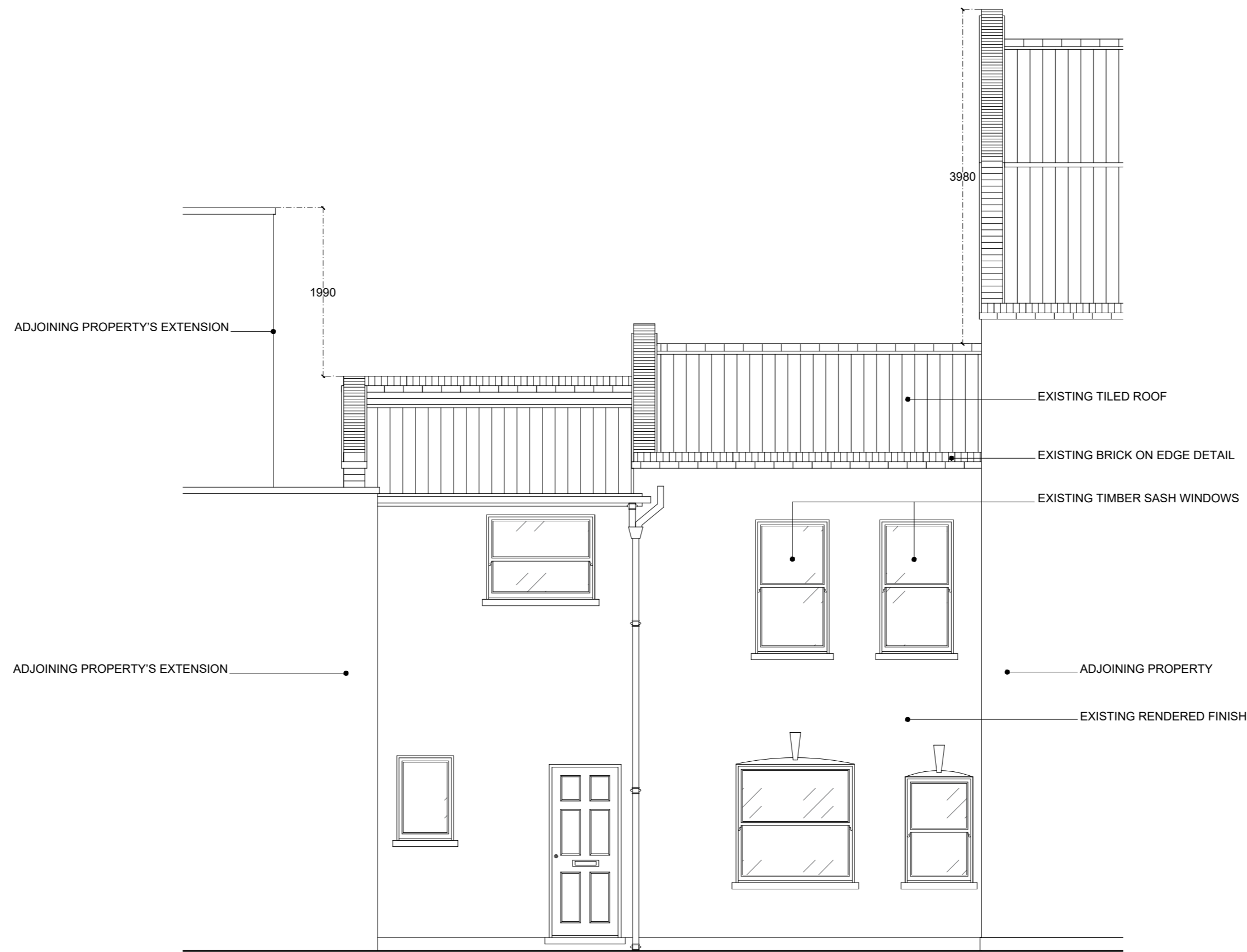
Z62 01 EXISTING | FRONT ELEVATION SHOWING ADJOINING PROPERTIES SCALE | 1:50 @ A2 / 1:100 @ A4
