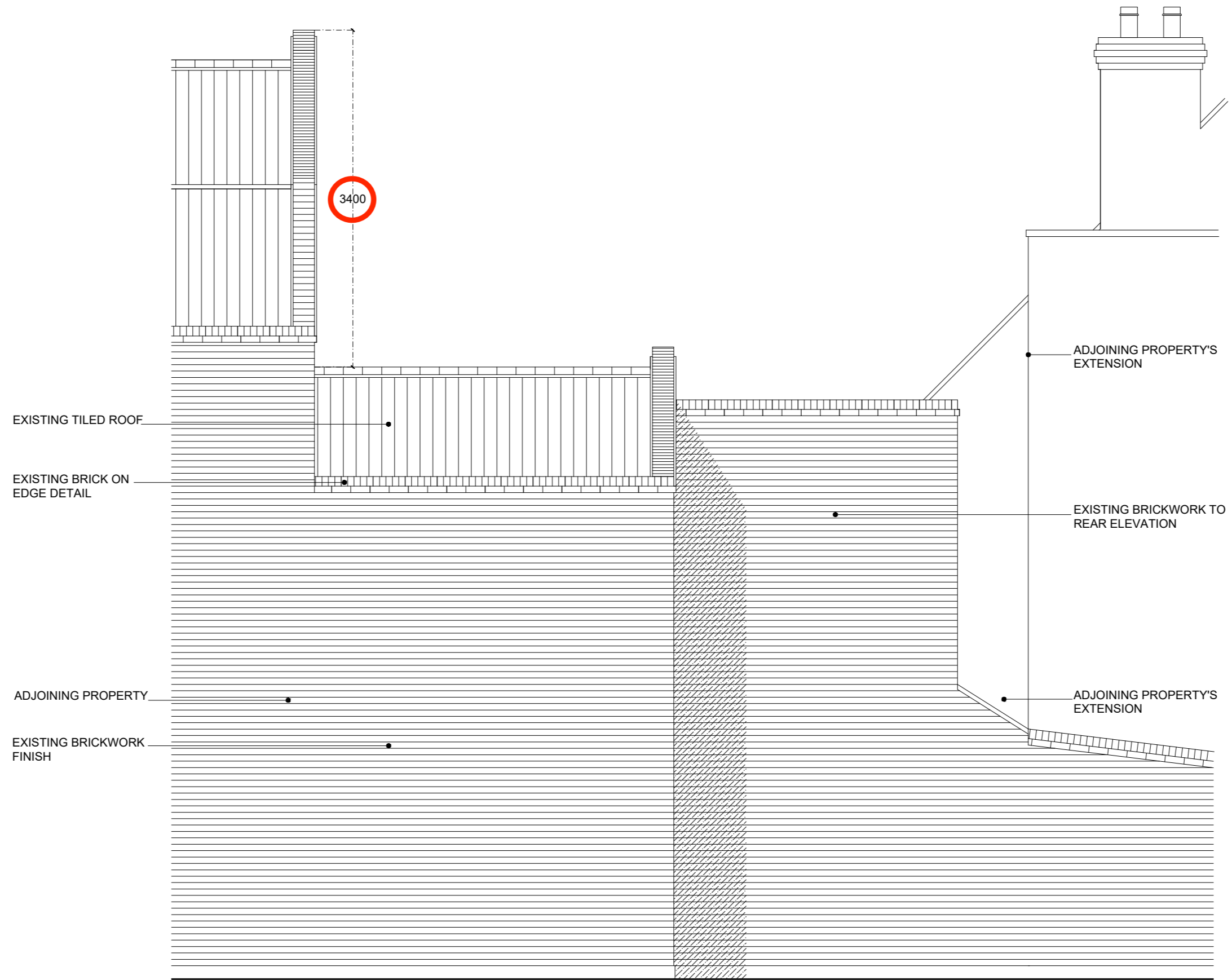
Z62 02 EXISTING | REAR ELEVATION SHOWING ADJOINING PROPERTIES SCALE | 1:50 @ A2 / 1:100 @ A4
