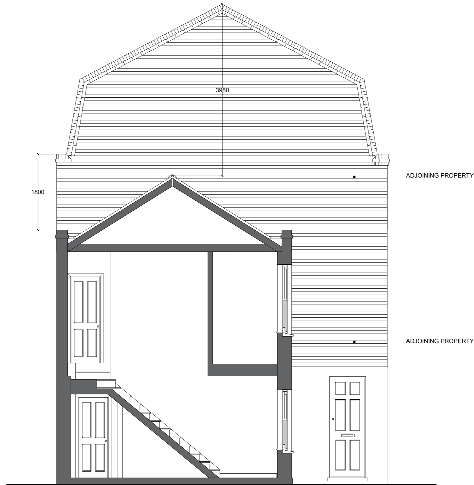
Z61 01 EXISTING | SECTION 01 SHOWING ADJOINING PROPERTIES SCALE | 1:50 @ A2 / 1:100 @ A4
