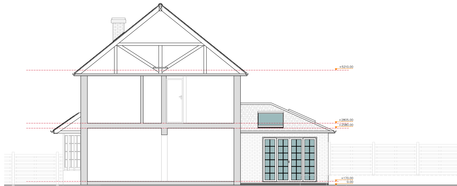
1 006 EXISTING SECTION SCALE 1:100
