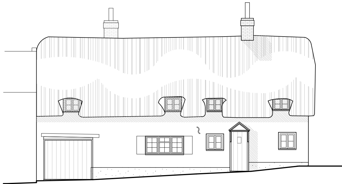
EAST ELEVATION 1:100 EXISTING
