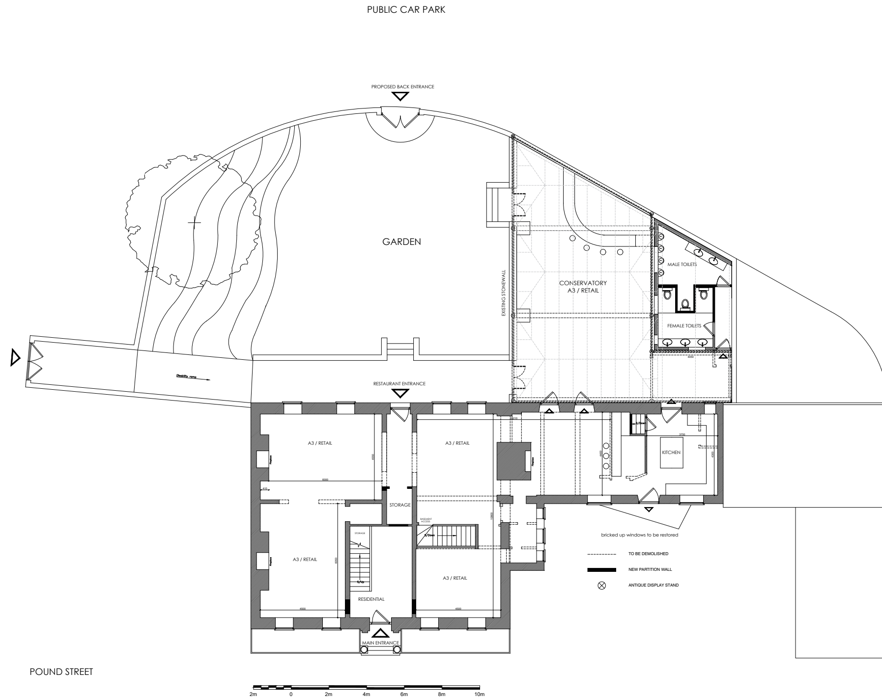
PROPOSED GROUND FLOOR PLAN - A3 / RETAIL / RESIDENTIAL ACCESS
