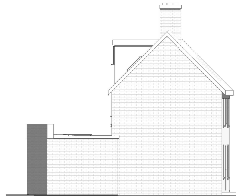
Proposed Elevation-Left side
