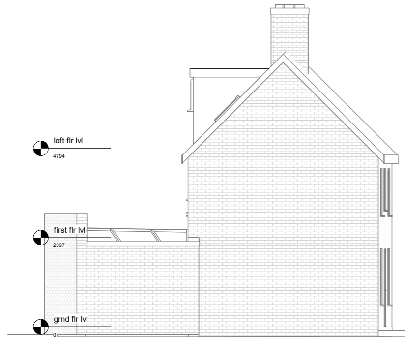
Existing Elevation-Left side
