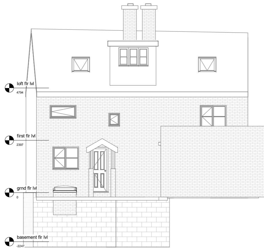
Existing Elevation-Rear
