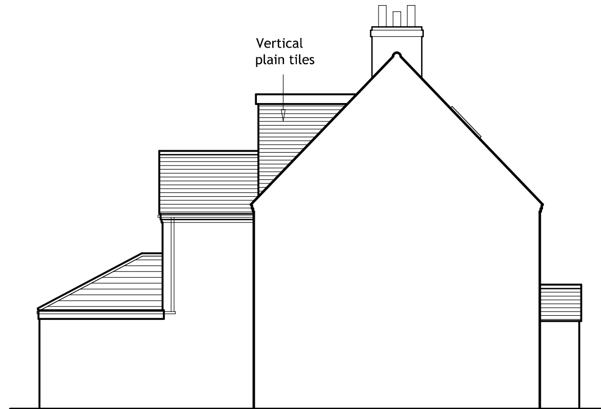
PROPOSED SIDE ELEVATION - THROUGH PARTY WALL -
