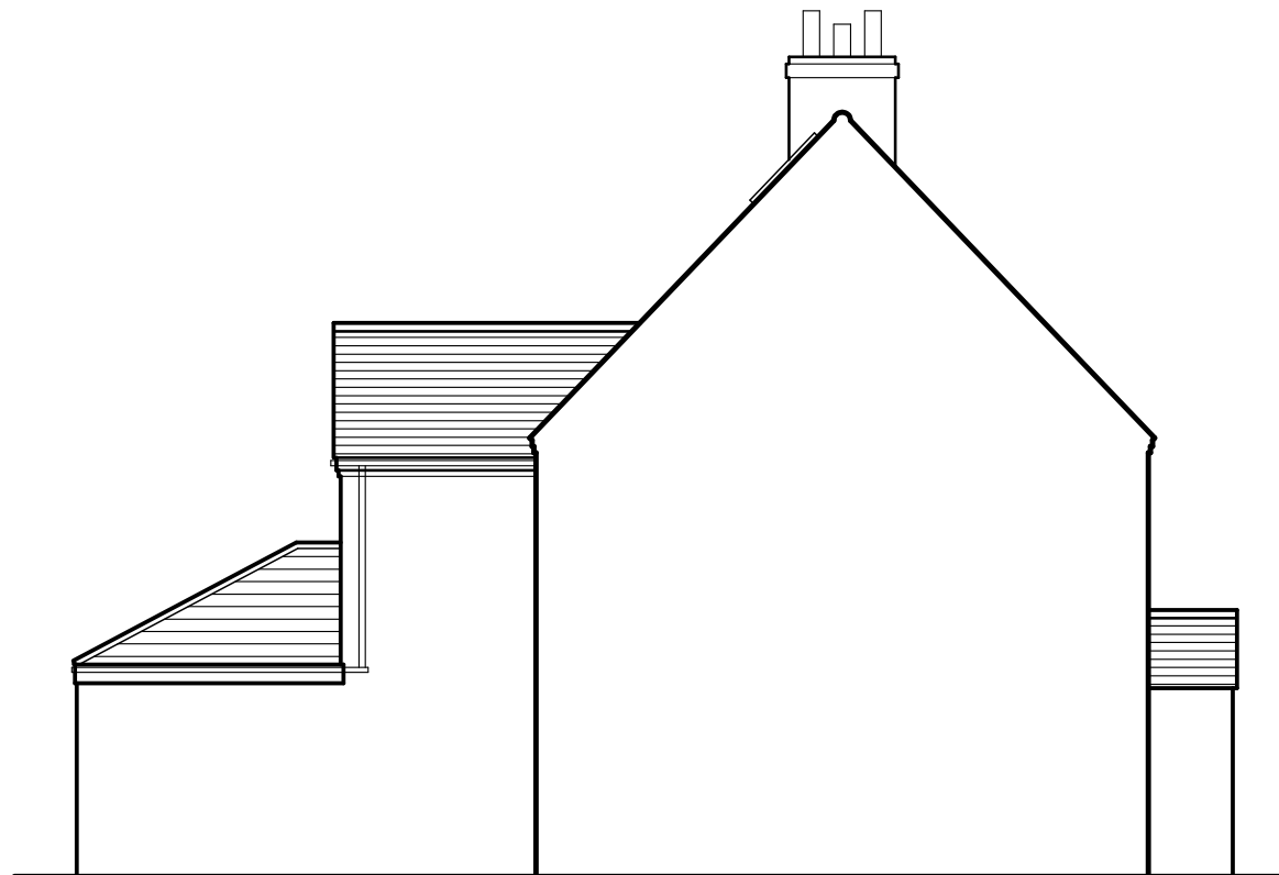
EXISTING SIDE ELEVATION - THROUGH PARTY WALL -
