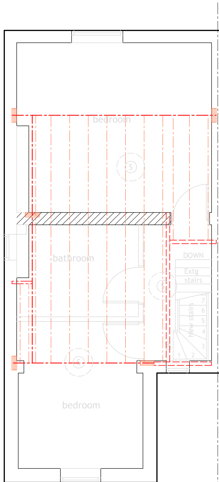
PROPOSED FIRST FLOOR PLAN - LOFT FLOOR CONSTRUCTION SUPERIMPOSED -
