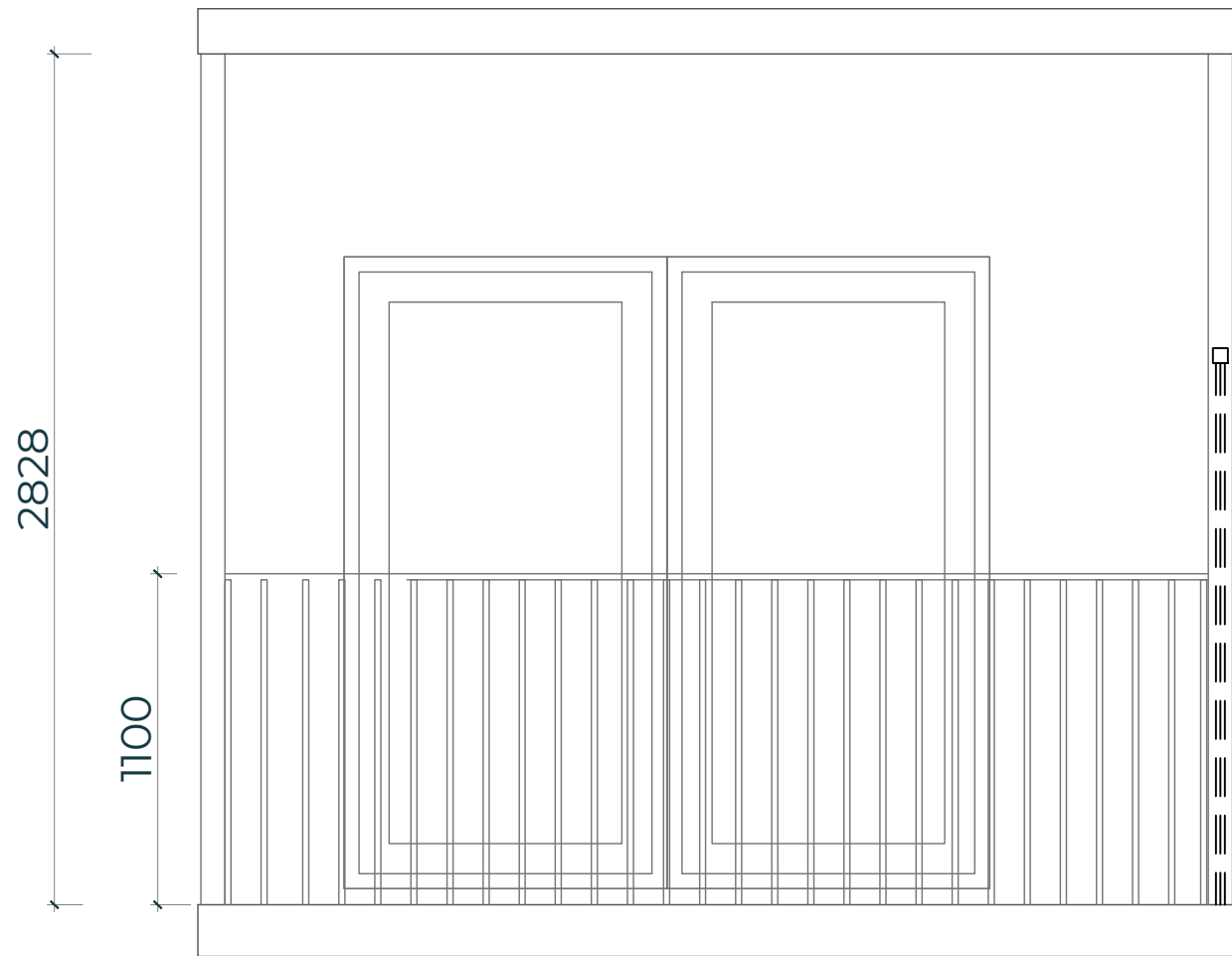
NORTH-EAST BALCONY - FRONT ELEVATION
